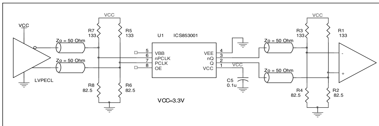
FIGURE 6. APPLICATION SCHEMATIC EXAMPLE
