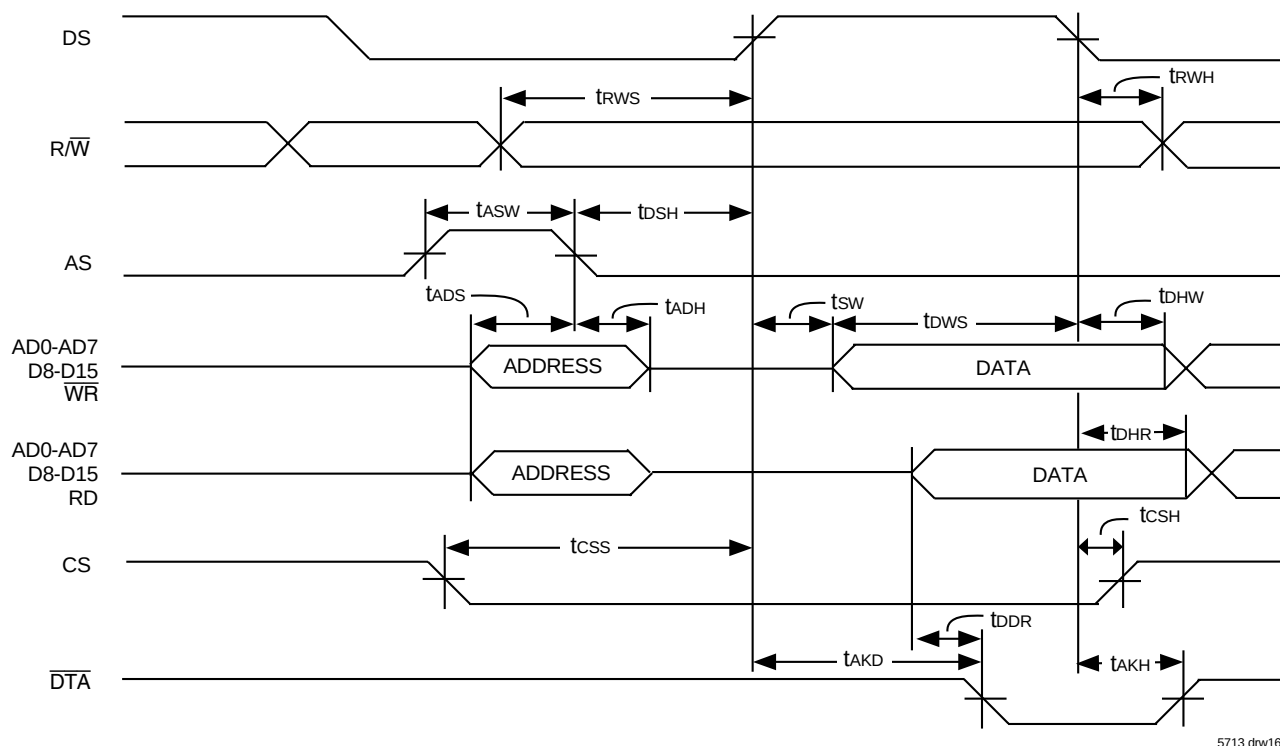
Figure 13. Multiplexed Bus Timing (Motorola Mode)
