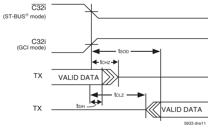
Figure 8. Serial Output and External Control
