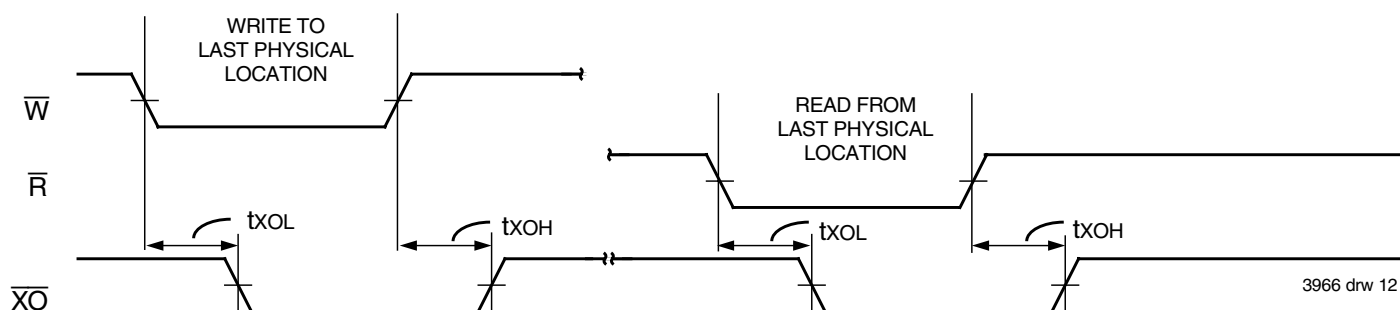
Figure 10. Expansion Out
