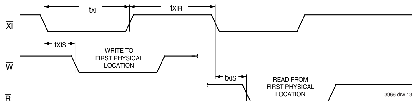
Figure 11. Expansion In
