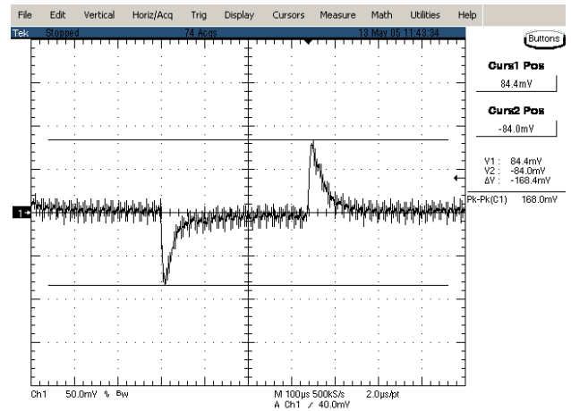
Figure 14: Typical transient response to step load change at 0.5\text{A}/\mu\text{S} from 50% to 100% of I_o , max at 36\text{V}_{in} , 6.5\text{V} out (measurement with a 1\mu\text{F} ceramic)
