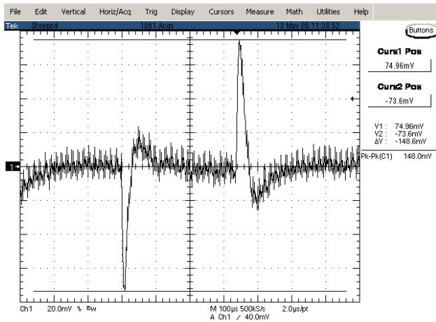
Figure 13: Typical transient response to step load change at 0.5\text{A}/\mu\text{S} from 100% to 50% of I_o , max at 24\text{V}_{in} , 15.0\text{V} out (measurement with a 1\mu\text{F} ceramic)
