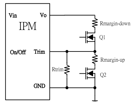
Figure 23: Circuit configuration for output voltage margining
