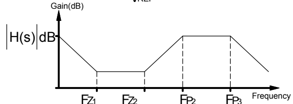
Fig.18: Compensation network with local feedback and its asymptotic gain plot
