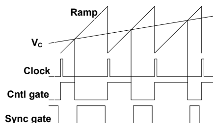
Fig. 7: Trailing-edge Modulation
