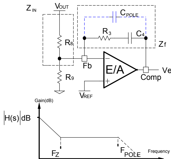
Fig. 17: Typell compensation gain network and its asymptotic gain plot
