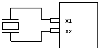
FIGURE 4. RECOMMENDED CRYSTAL CONNECTION
