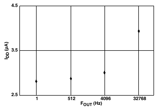
FIGURE 6. I_{DD1} vs f_{OUT} AT V_{DD} = 5V
