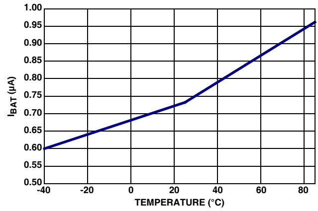
FIGURE 2. I_{BAT} vs TEMPERATURE AT V_{BAT} = 3V
