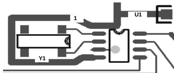
FIGURE 19. SUGGESTED LAYOUT FOR ISL12082 AND CRYSTAL
