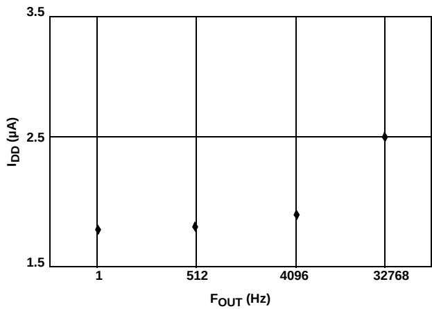
FIGURE 5. I_{DD1} vs f_{OUT} AT V_{DD} = 3.3V
