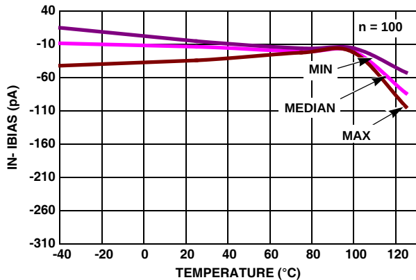
FIGURE 41. I BIAS(IN-) vs TEMPERATURE V_S = \pm 1.2V
