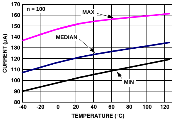
FIGURE 27. TOTAL SUPPLY CURRENT vs TEMPERATURE V_S = \pm 2.5V ENABLED. R_L = \infty
