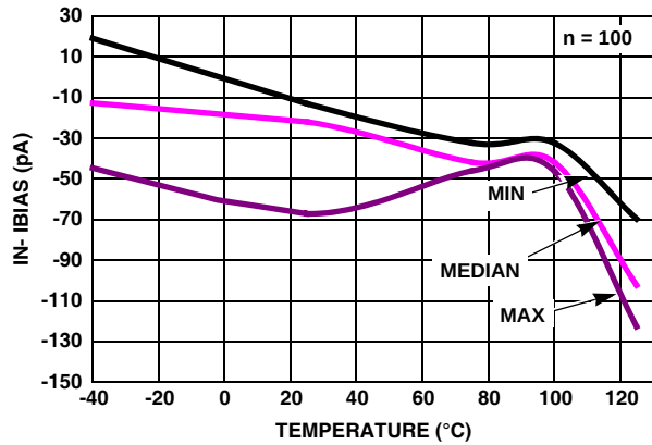
FIGURE 39. I BIAS(IN-) vs TEMPERATURE V_S = \pm 2.5V
