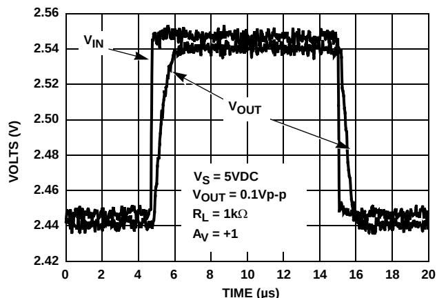
FIGURE 19. AMPLIFIER "B" (OP-AMP) SMALL SIGNAL TRANSIENT RESPONSE
