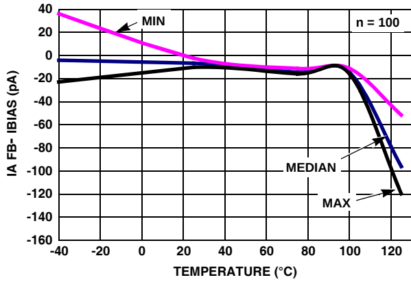
FIGURE 31. I BIAS (IA FB-) vs TEMPERATURE V_S = \pm 2.5V .
