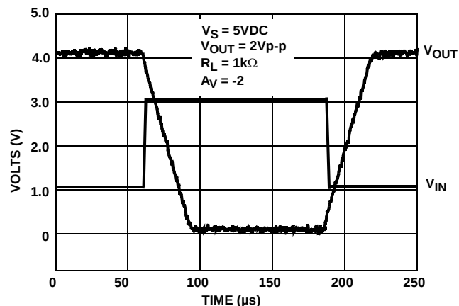
FIGURE 20. AMPLIFIER "B" (OP-AMP) LARGE SIGNAL TRANSIENT RESPONSE
