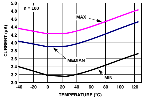
FIGURE 28. DISABLED POSITIVE SUPPLY CURRENT vs TEMPERATURE V_S = \pm 2.5V . R_L = \infty
