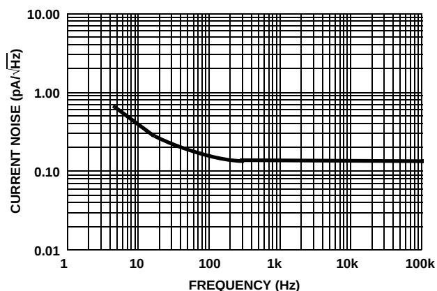
FIGURE 21. AMPLIFIER "B" (OP-AMP) CURRENT NOISE vs FREQUENCY
