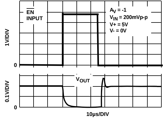
FIGURE 26. AMPLIFIER "B" (OP-AMP) ENABLE TO OUTPUT DELAY TIME
