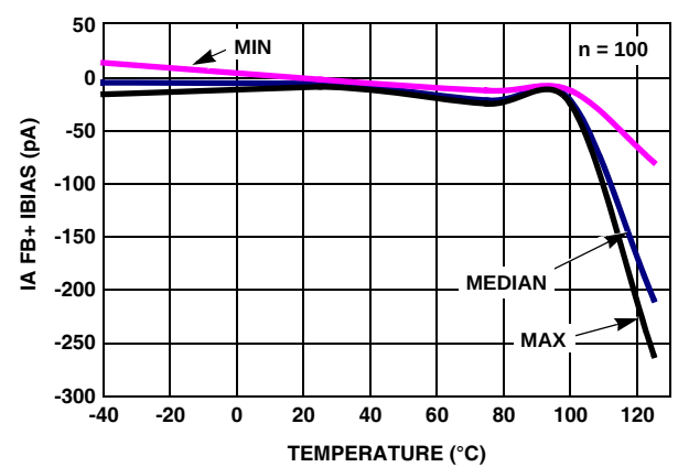
FIGURE 30. IBIAS ( I_A FB+) vs TEMPERATURE V_S = \pm 2.5V .
