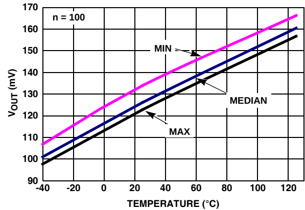
FIGURE 60. V_{OUT} LOW vs TEMPERATURE R_L = 1k . V_S = \pm 2.5V
