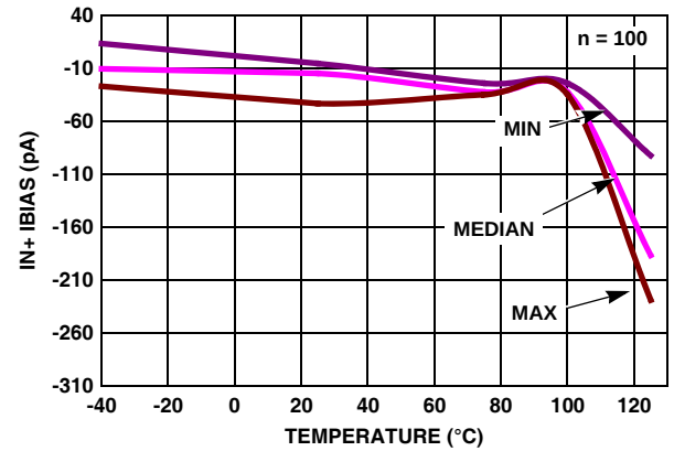
FIGURE 40. I BIAS(IN+) vs TEMPERATURE V_S = \pm 1.2V
