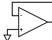
FIGURE 65. PREVENTING OSCILLATIONS IN UNUSED CHANNELS
