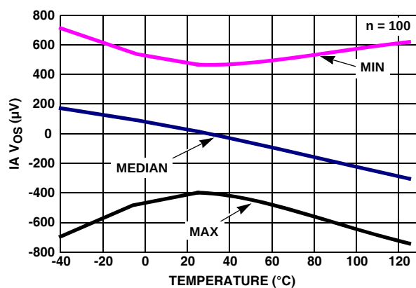
FIGURE 46. IA INPUT OFFSET VOLTAGE vs TEMPERATURE V_S = \pm 2.5V
