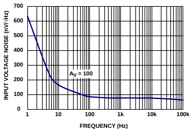
FIGURE 8. AMPLIFIER "A"(INAMP) INPUT VOLTAGE NOISE SPECTRAL DENSITY
