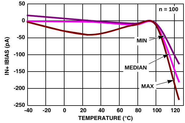
FIGURE 38. I BIAS(IN+) vs TEMPERATURE V_S = \pm 2.5V
