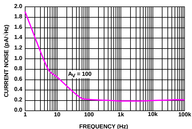
FIGURE 9. AMPLIFIER "A"(INAMP) INPUT CURRENT NOISE SPECTRAL DENSITY
