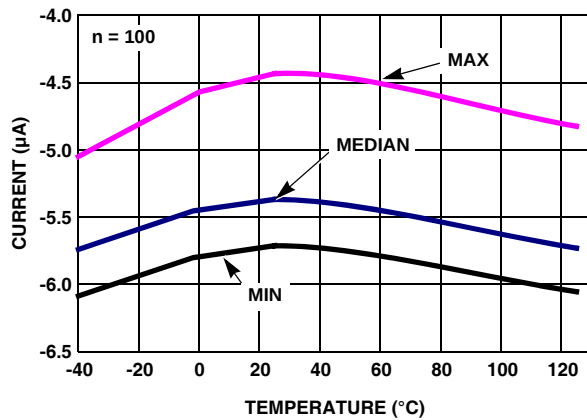
FIGURE 29. DISABLED NEGATIVE SUPPLY CURRENT vs TEMPERATURE V_S = \pm 2.5V . R_L = \infty
