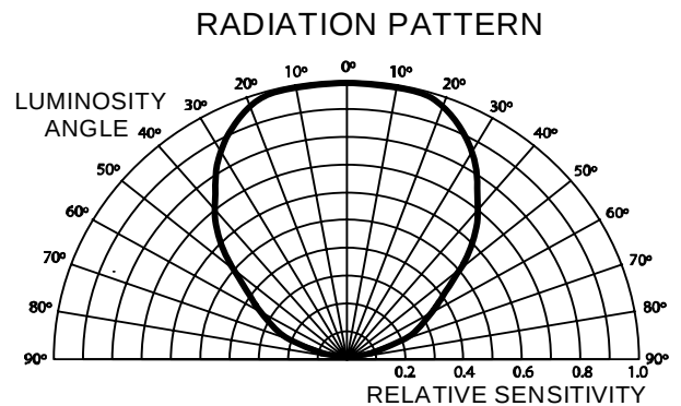
FIGURE 10. RADIATION PATTERN
