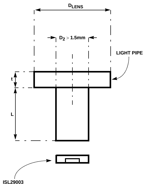
FIGURE 5. WINDOW WITH LIGHT GUIDE/PIPE
