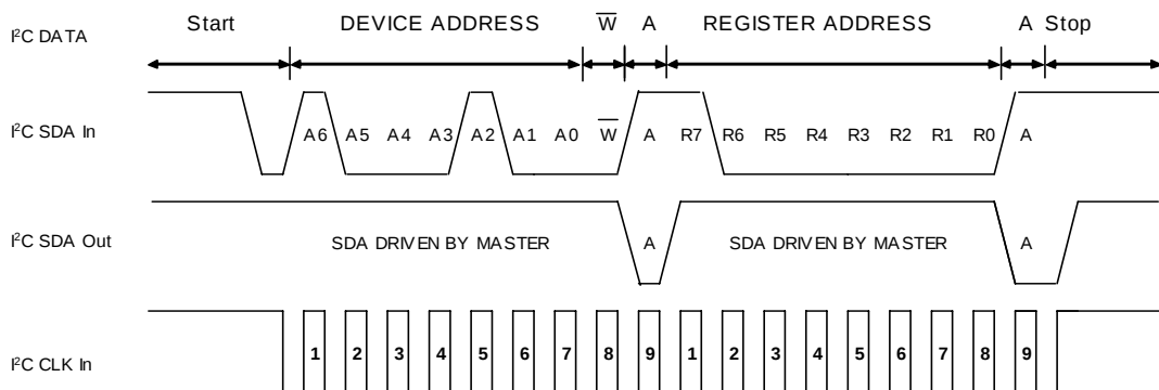
FIGURE 3. I²C sync_iic TIMING DIAGRAM SAMPLE
