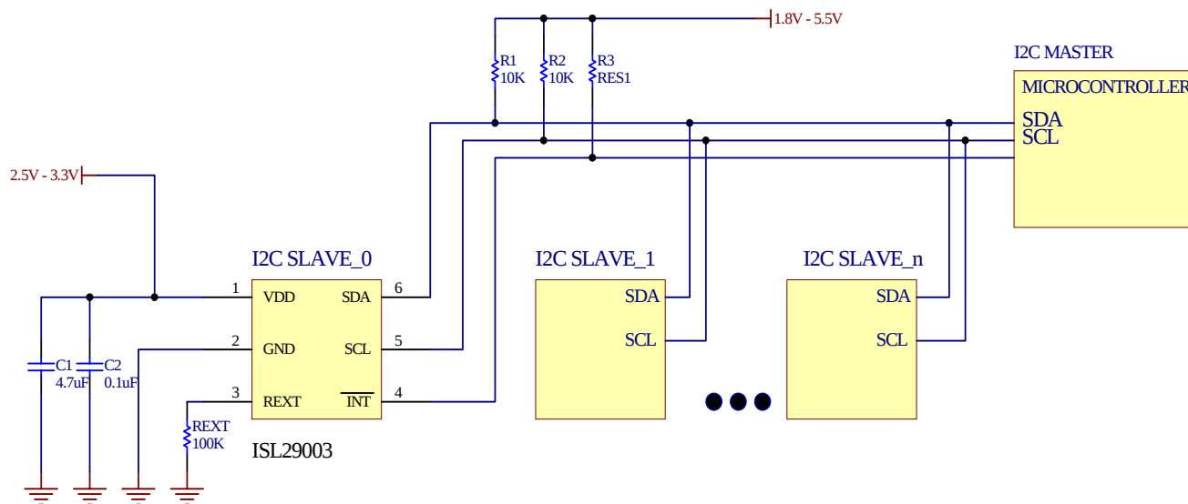
FIGURE 6. ISL29003 TYPICAL CIRCUIT
