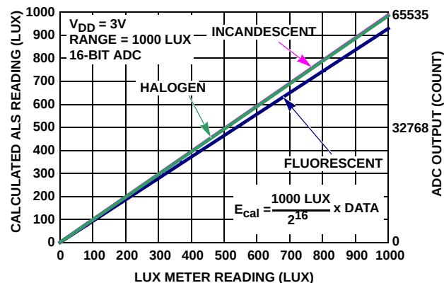
FIGURE 8. SENSITIVITY TO FOUR LIGHT SOURCES
