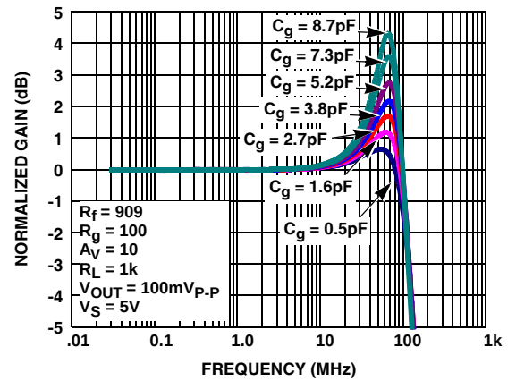
FIGURE 8. ISL55291 GAIN vs FREQUENCY FOR VARIOUS C_g
