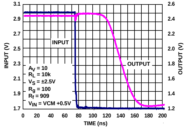
FIGURE 22. ISL55291 POSITIVE INPUT RECOVERY TIME
