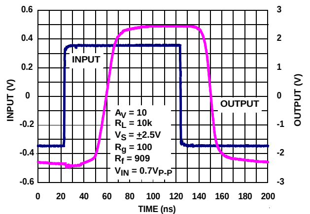
FIGURE 24. OUTPUT OVERLOAD RECOVERY
