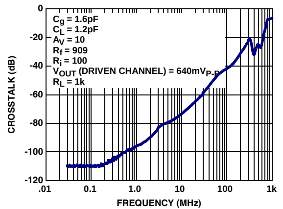
FIGURE 16. ISL55291 CHANNEL TO CHANNEL CROSSTALK vs FREQUENCY
