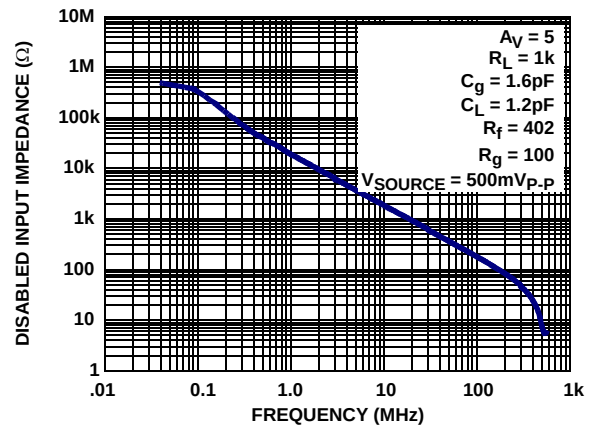
FIGURE 10. DISABLED INPUT IMPEDANCE vs FREQUENCY
