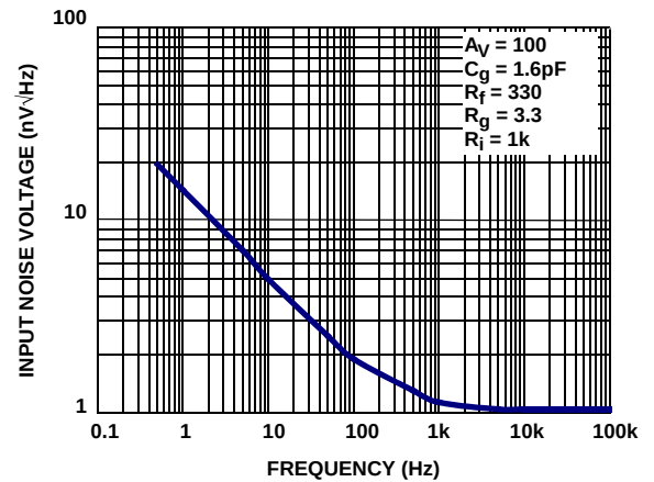
FIGURE 18. INPUT VOLTAGE NOISE vs FREQUENCY
