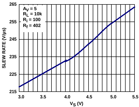
FIGURE 27. ISL55290 POSITIVE SLEW RATE vs VS
