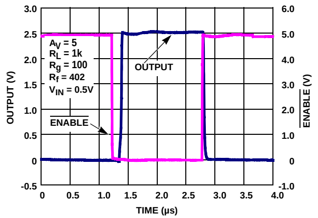
FIGURE 26. ISL55290 ENABLE TO OUTPUT DELAY
