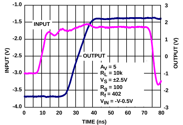
FIGURE 24. NEGATIVE INPUT OVERLOAD RECOVERY TIME
