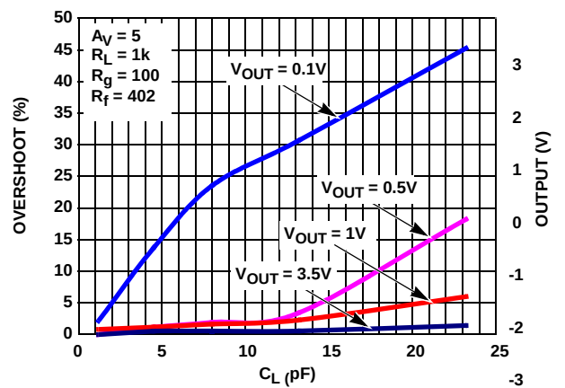
FIGURE 22. ISL55290 PERCENT OVERSHOOT vs V_{OUT} , C_L
