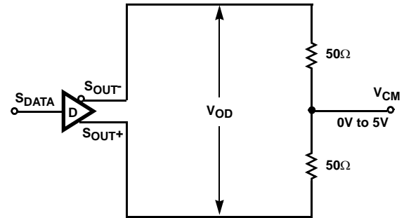
FIGURE 1B. V_{OD} WITH COMMON MODE LOAD
