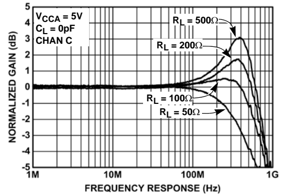
FIGURE 8. DIFFERENTIAL FREQUENCY RESPONSE FOR VARIOUS R_L - DIFF (CHANNEL C)
