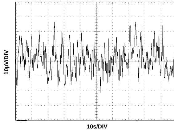
FIGURE 27. V_{OUT} NOISE
