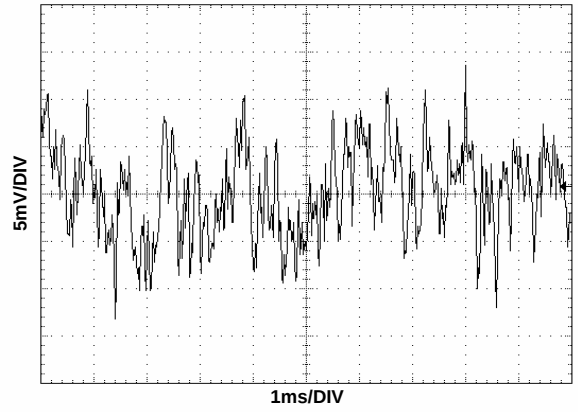
FIGURE 55. V_{OUT} NOISE
