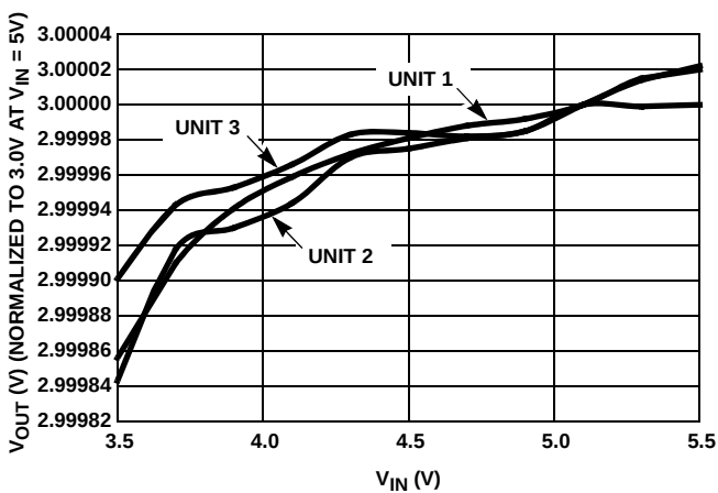
FIGURE 86. LINE REGULATION (3 REPRESENTATIVE UNITS)
