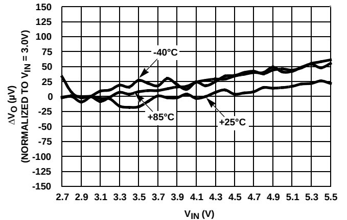
FIGURE 4. LINE REGULATION OVER TEMPERATURE
