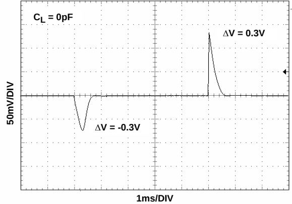
FIGURE 62. LINE TRANSIENT RESPONSE
