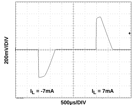
FIGURE 24. LOAD TRANSIENT RESPONSE
