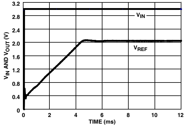
FIGURE 67. TURN-ON TIME ( +25^\circ C )
