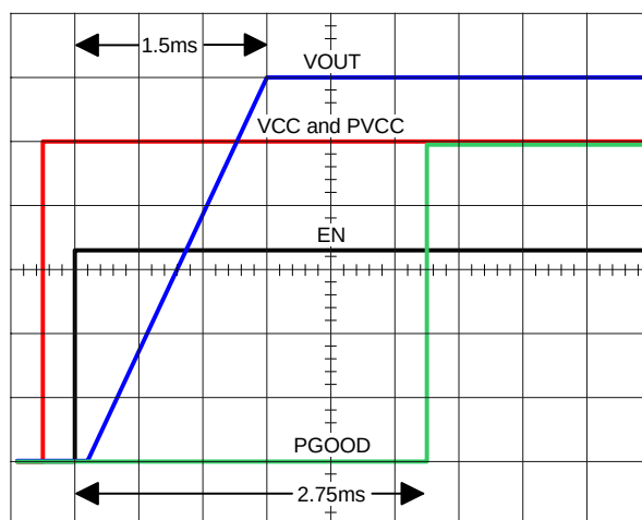
FIGURE 3. SOFT-START SEQUENCE
