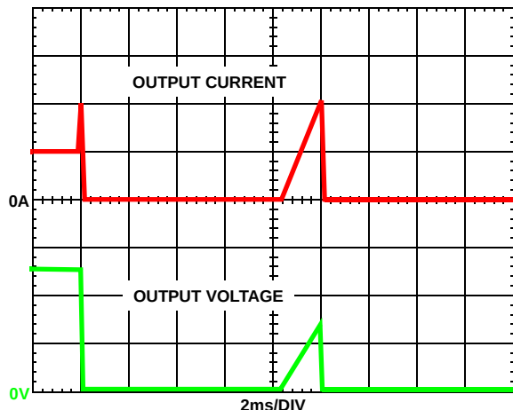
FIGURE 11. OVERCURRENT BEHAVIOR IN HICCUP MODE. F_{SW} = 500\text{kHz}
