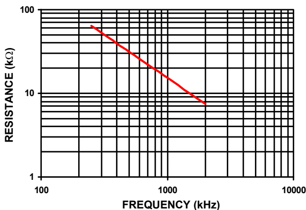
FIGURE 4. R_{FS} RESISTANCE vs. FREQUENCY
