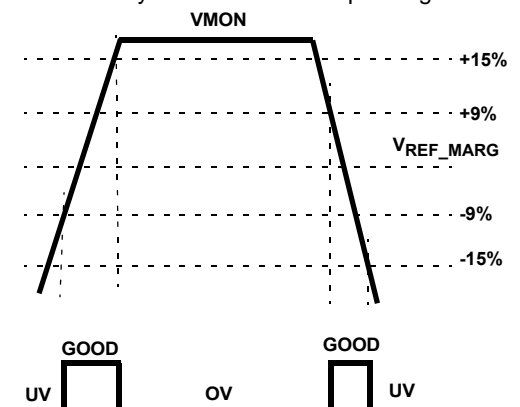
FIGURE 3. UNDERVOLTAGE-OVERVOLTAGE WINDOW
