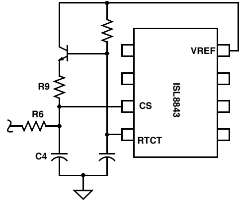
FIGURE 6. SLOPE COMPENSATION
