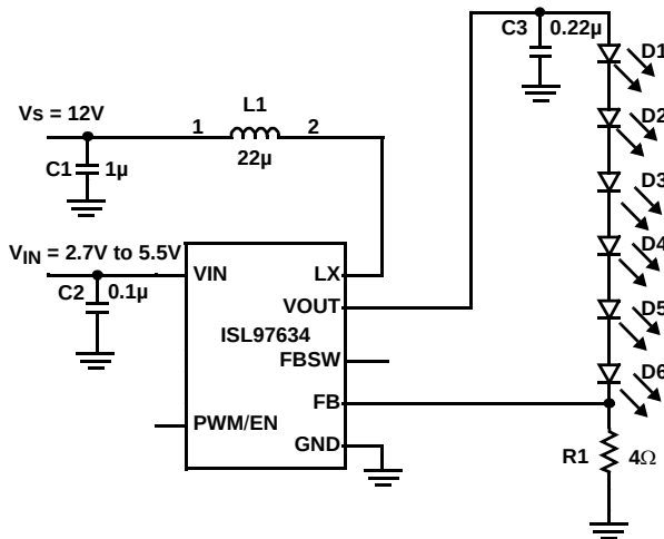
FIGURE 15. SEPARATE HIGH INPUT VOLTAGE FOR HIGHER EFFICIENCY OPERATION
