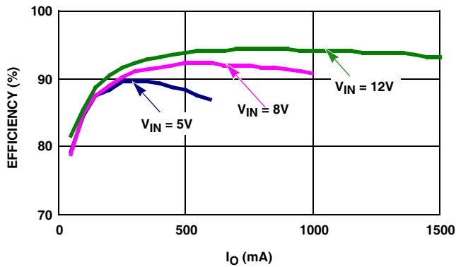
FIGURE 1. BOOST EFFICIENCY
