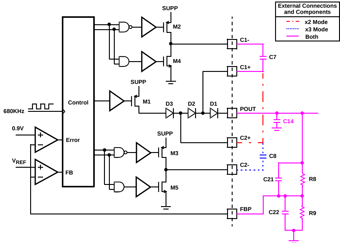
FIGURE 16. V_{ON} FUNCTION DIAGRAM
