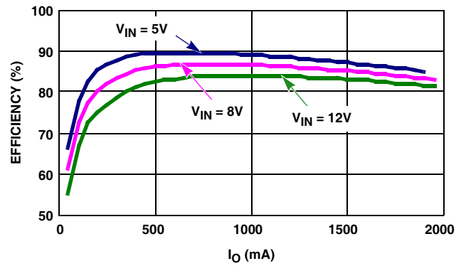
FIGURE 4. BUCK EFFICIENCY
