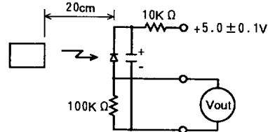
Fig. 2 STD. TRANSMITTER TEST CIRCUIT
