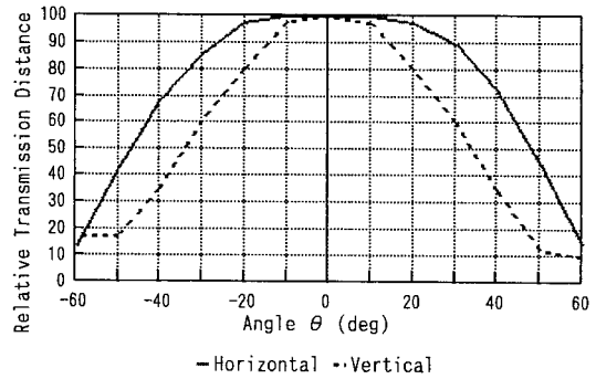
Directivity ( T_a=25^\circ\text{C} )
