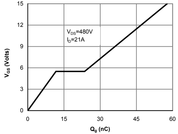
Figure 8: Gate-Charge Characteristics
