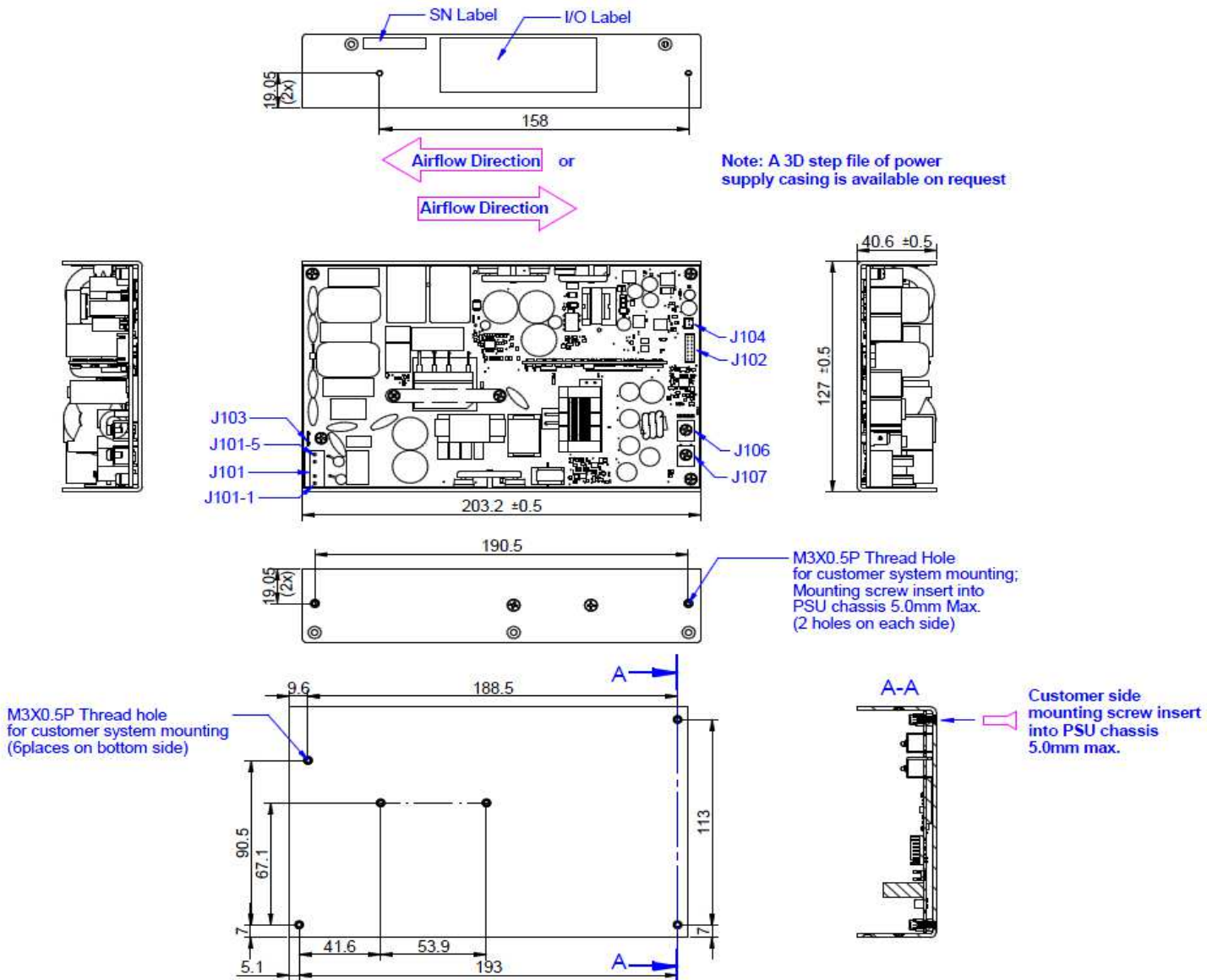
Figure 7: Dimensions Drawing
