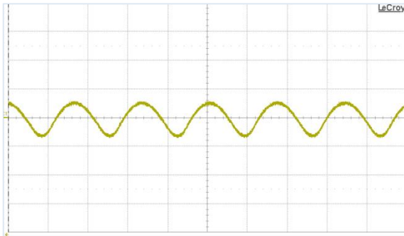
Fig. 15: Input reflected ripple current, i_c (2 A/div.), measured at input terminals at full rated load current and V_{in} = 48 \text{ V} . Refer to Fig. 14 for test setup. Time scale: 2 \mu\text{s}/\text{div} .
