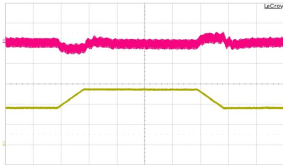
Fig. 11: Output voltage response to load current step change (36 A - 54 A - 36 A) at V_{in} = 48\text{ V} . Top trace: output voltage (200 mV/div.). Bottom trace: load current (20 A/div.). Current slew rate: 0.1 A/ \mu\text{s} . C_o = 1\ \mu\text{F} ceramic + 10 \mu\text{F} tantalum. Time scale: 200 \mu\text{s} /div.
