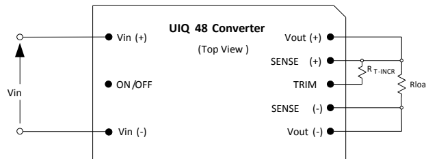
Fig. C: Configuration for increasing output voltage.
