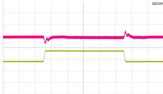
Fig. 12: Output voltage response to load current step change (36 A - 54 A - 36 A) at V_{in} = 48\text{ V} . Top trace: output voltage (500 mV/div.). Bottom trace: load current (20 A/div.). Current slew rate: 1 A/ \mu\text{s} . C_o = 1\ \mu\text{F} ceramic + 10,000 \mu\text{F} tantalum. Time scale: 200 \mu\text{s} /div.
