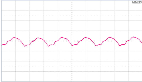
Fig. 13: Output voltage ripple (50 mV/div.) at full rated load current C_o = 10 \mu\text{F} tantalum + 1 \mu\text{F} ceramic and V_{in} = 48 \text{ V} . Time scale: 2 \mu\text{s}/\text{div} .
