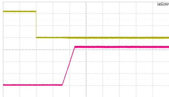
Fig. 10: Turn-on transient at full rated load current (resistive) plus 10,000 \mu\text{F} at V_{in} = 48\text{ V} , triggered via ON/OFF pin. Top trace: ON/OFF signal (2 V/div.). Bottom trace: output voltage (1 V/div.). Time scale: 50 ms/div.
