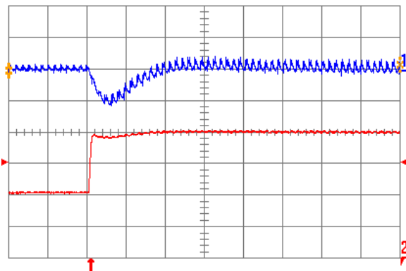
Fig. 2.5V.6: Output voltage response for V_{out} = 2.5 V to positive load current step change from 10 A to 20 A with slew rate of 5\text{A}/\mu\text{s} at V_{in} = 12 V. Top trace: output voltage (200 mV/div.); Bottom trace: load current (5 A/div.). C_o = 100 \mu\text{F} ceramic. Time scale: 20 \mu\text{s} /div.
