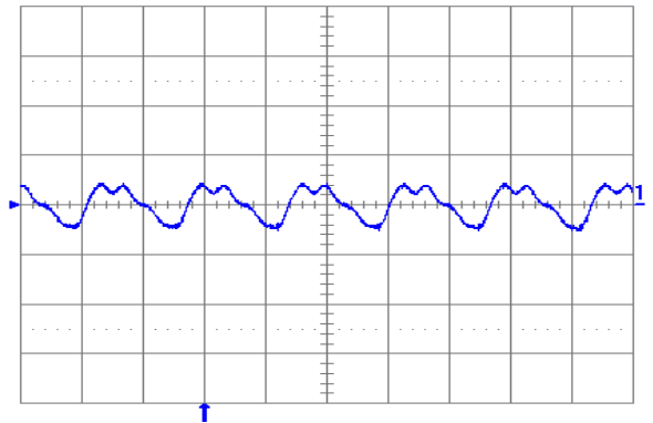
Fig. 2.5V.5: Output voltage ripple (20 mV/div.) at full rated load current into a resistive load with external capacitance 100 \mu\text{F} ceramic + 1 \mu\text{F} ceramic and V_{in} = 12 V for V_{out} = 2.5 V. Time scale: 2 \mu\text{s} /div.
