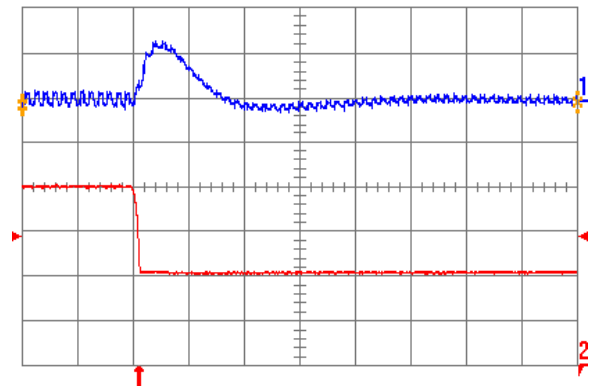
Fig. 5.0V.7: Output voltage response for V_{out} = 5.0 V to negative load current step change from 20 A to 10 A with slew rate of -5 \text{ A}/\mu\text{s} at V_{in} = 12 V. Top trace: output voltage (200 mV/div.); Bottom trace: load current (5 A/div.). C_o = 100 \mu\text{F} ceramic. Time scale: 20 \mu\text{s} /div.
