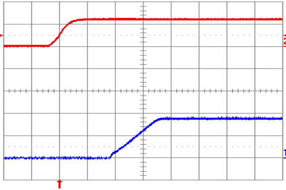
Fig. 1.8V.4: Turn-on transient for V_{out} = 1.8 V with application of V_{in} at full rated load current (resistive) and 100 \mu\text{F} external capacitance at V_{in} = 12 V. Top trace: V_{in} (10 V/div.); Bottom trace: output voltage (1 V/div.); Time scale: 2 ms/div.
