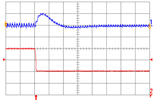
Fig. 2.5V.7: Output voltage response for V_{out} = 2.5 V to negative load current step change from 20 A to 10 A with slew rate of -5\text{A}/\mu\text{s} at V_{in} = 12 V. Top trace: output voltage (200 mV/div.); Bottom trace: load current (5 A/div.). C_o = 100 \mu\text{F} ceramic. Time scale: 20 \mu\text{s} /div.
