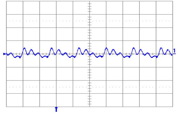
Fig. 1.5V.5: Output voltage ripple (20 mV/div.) at full rated load current into a resistive load with external capacitance 100 \mu\text{F} ceramic + 1 \mu\text{F} ceramic and V_{in} = 12 V for V_{out} = 1.5 V. Time scale: 2 \mu\text{s} /div.
