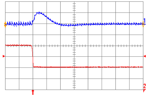
Fig. 1.8V.7: Output voltage response for V_{out} = 1.8 V to negative load current step change from 20 A to 10 A with slew rate of -5 \text{ A}/\mu\text{s} at V_{in} = 12 V. Top trace: output voltage (200 mV/div.); Bottom trace: load current (5 A/div.). C_o = 100 \mu\text{F} ceramic. Time scale: 20 \mu\text{s} /div.
