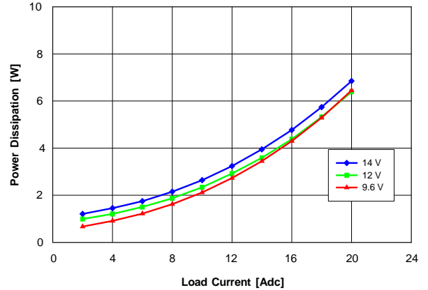
Fig. 5.0V.3: Power loss vs. load current and input voltage for V_{out} = 5.0\text{ V} converter mounted vertically with air flowing at a rate of 200 LFM (1 m/s) and T_a = 25\text{ }^{\circ}\text{C} .
