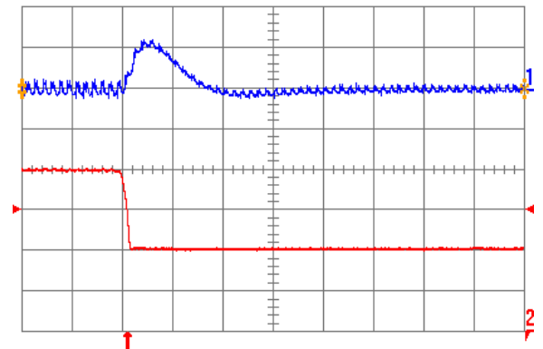
Fig. 3.3V.7: Output voltage response for V_{out} = 3.3 V to negative load current step change from 20 A to 10 A with slew rate of -5 \text{ A}/\mu\text{s} at V_{in} = 12 V. Top trace: output voltage (200 mV/div.); Bottom trace: load current (5 A/div.). C_o = 100 \mu\text{F} ceramic. Time scale: 20 \mu\text{s} /div.
