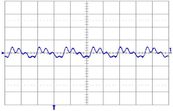
Fig. 1.8V.5: Output voltage ripple (20 mV/div.) at full rated load current into a resistive load with external capacitance 100 \mu\text{F} ceramic + 1 \mu\text{F} ceramic and V_{in} = 12 V for V_{out} = 1.8 V. Time scale: 2 \mu\text{s} /div.
