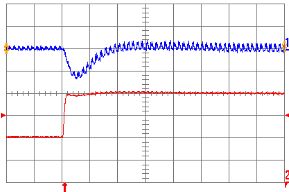
Fig. 3.3V.6: Output voltage response for V_{out} = 3.3 V to positive load current step change from 10 A to 20 A with slew rate of 5 \text{ A}/\mu\text{s} at V_{in} = 12 V. Top trace: output voltage (200 mV/div.); Bottom trace: load current (5 A/div.). C_o = 100 \mu\text{F} ceramic. Time scale: 20 \mu\text{s} /div.
