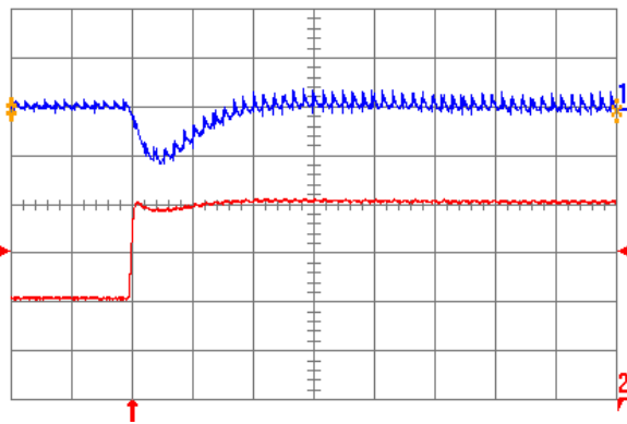
Fig. 1.8V.6: Output voltage response for V_{out} = 1.8 V to positive load current step change from 10 A to 20 A with slew rate of 5 \text{ A}/\mu\text{s} at V_{in} = 12 V. Top trace: output voltage (200 mV/div.); Bottom trace: load current (5 A/div.). C_o = 100 \mu\text{F} ceramic. Time scale: 20 \mu\text{s} /div.
