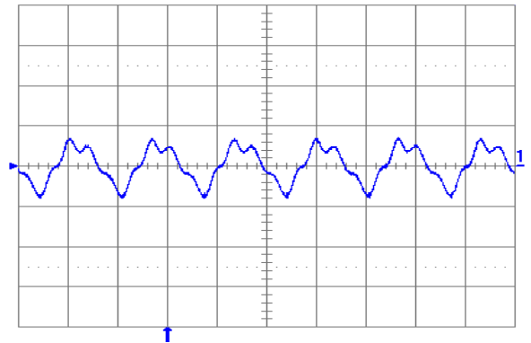
Fig. 3.3V.5: Output voltage ripple (20 mV/div.) at full rated load current into a resistive load with external capacitance 100 \mu\text{F} ceramic + 1 \mu\text{F} ceramic and V_{in} = 12 V for V_{out} = 3.3 V. Time scale: 2 \mu\text{s} /div.
