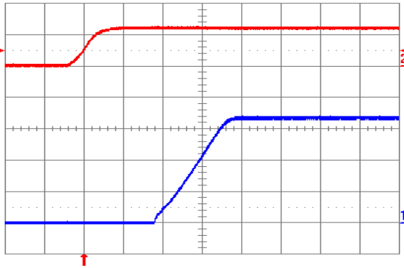
Fig. 3.3V.4: Turn-on transient for V_{out} = 3.3 V with application of V_{in} at full rated load current (resistive) and 100 \mu\text{F} external capacitance at V_{in} = 12 V. Top trace: V_{in} (10 V/div.); Bottom trace: output voltage (1 V/div.); Time scale: 2 ms/div.
