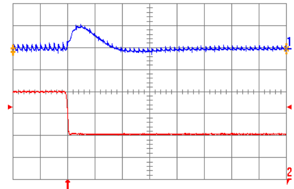
Fig. 1.5V.7: Output voltage response for V_{out} = 1.5 V to negative load current step change from 20 A to 10 A with slew rate of -5 \text{ A}/\mu\text{s} at V_{in} = 12 V. Top trace: output voltage (200 mV/div.); Bottom trace: load current (5 A/div.). C_o = 100 \mu\text{F} ceramic. Time scale: 20 \mu\text{s} /div.
