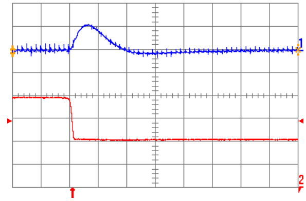
Fig. 0.7525V.7: Output voltage response for V_{out} = 0.7525 V to negative load current step change from 20 A to 10 A with slew rate of -5\text{A}/\mu\text{s} at V_{in} = 12 V. Top trace: output voltage (200 mV/div.); Bottom trace: load current (5 A/div.). C_o = 100 \mu\text{F} ceramic. Time scale: 20 \mu\text{s}/\text{div} .
