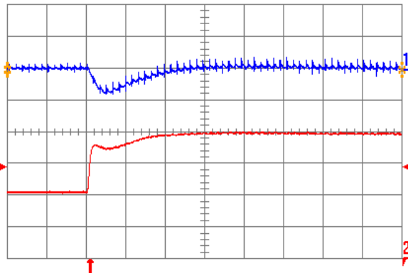
Fig. 0.7525V.6: Output voltage response for V_{out} = 0.7525 V to positive load current step change from 10 A to 20 A with slew rate of 5\text{A}/\mu\text{s} at V_{in} = 12 V. Top trace: output voltage (200 mV/div.); Bottom trace: load current (5 A/div.). C_o = 100 \mu\text{F} ceramic. Time scale: 20 \mu\text{s}/\text{div} .
