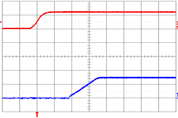
Fig. 1.5V.4: Turn-on transient for V_{out} = 1.5 V with application of V_{in} at full rated load current (resistive) and 100 \mu\text{F} external capacitance at V_{in} = 12 V. Top trace: V_{in} (10 V/div.); Bottom trace: output voltage (1 V/div.); Time scale: 2 ms/div.
