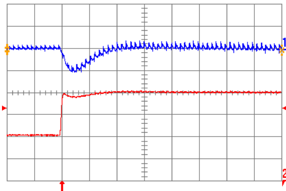
Fig. 1.5V.6: Output voltage response for V_{out} = 1.5 V to positive load current step change from 10 A to 20 A with slew rate of 5 \text{ A}/\mu\text{s} at V_{in} = 12 V. Top trace: output voltage (200 mV/div.); Bottom trace: load current (5 A/div.). C_o = 100 \mu\text{F} ceramic. Time scale: 20 \mu\text{s} /div.
