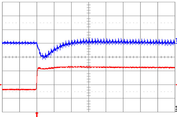
Fig. 2.0V.6: Output voltage response for V_{out} = 2.0 V to positive load current step change from 10 A to 20 A with slew rate of 5 \text{ A}/\mu\text{s} at V_{in} = 12 V. Top trace: output voltage (200 mV/div.); Bottom trace: load current (5 A/div.). C_o = 100 \mu\text{F} ceramic. Time scale: 20 \mu\text{s} /div.
