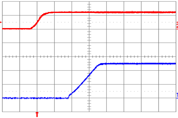
Fig. 2.5V.4: Turn-on transient for V_{out} = 2.5 V with application of V_{in} at full rated load current (resistive) and 100 \mu\text{F} external capacitance at V_{in} = 12 V. Top trace: V_{in} (10 V/div.); Bottom trace: output voltage (1 V/div.); Time scale: 2 ms/div.
