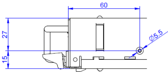
Figure 38 - PFE3000-12-069RA with Key-in screw dimension (Option code S366)
