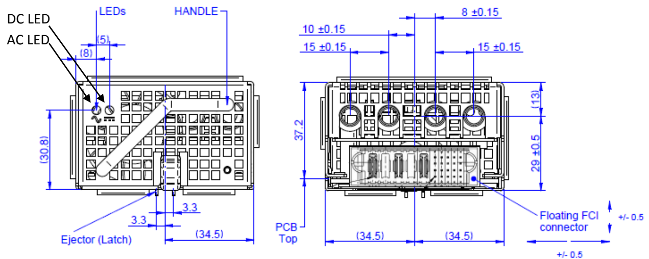
Figure 37 - Front and rear view
