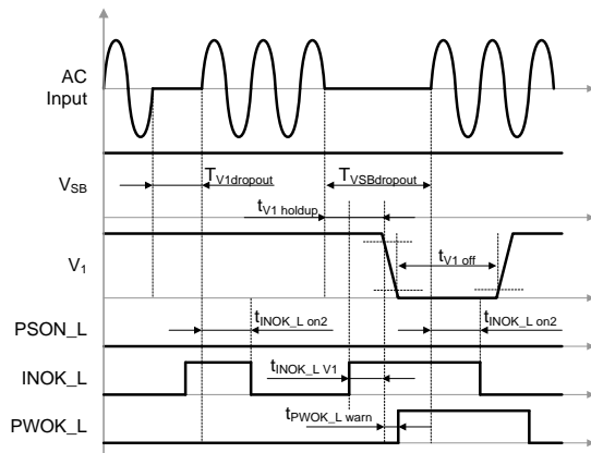
Figure 24 - AC short dips
