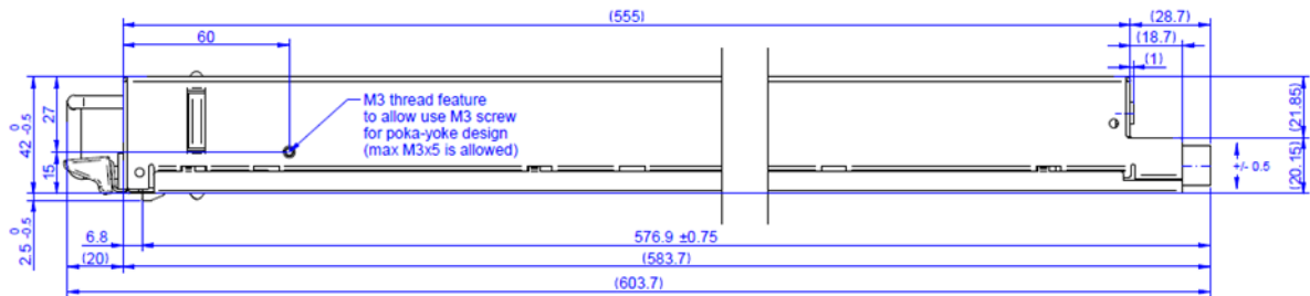
Figure 36 - Top view
