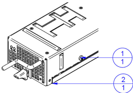
Figure 39 - PFE3000-12-069RA with Key-in screw (Option code S366)
