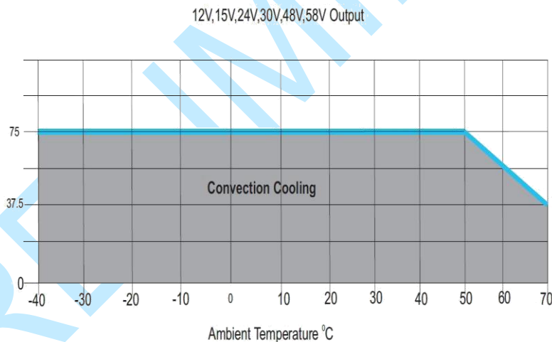
Figure 1 – Derating Curve
