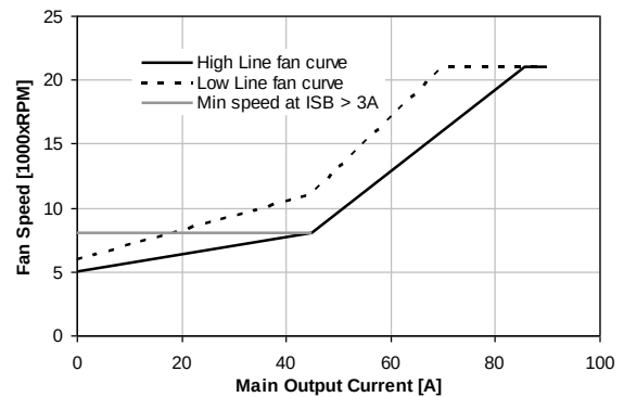
Figure 40 - Fan speed vs. main output load for PFE1100-12-054RA
