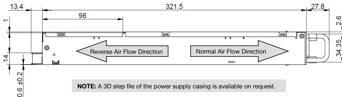
Figure 43 - Side View 1
