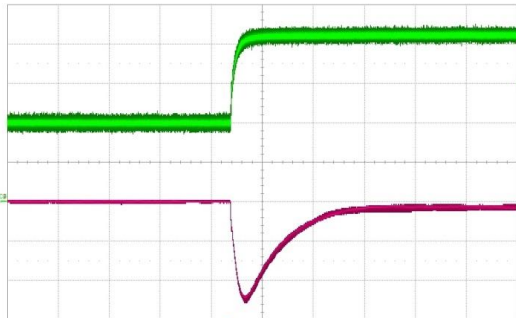
Figure 17 - Load transient V_1 , 40 to 85A (500μs/div) CH2: V_1 (200mV/div) CH4: I_1 (20A/div)
