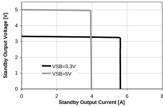
Figure 22 - Current limitation on V_{SB}
