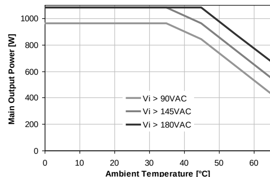
Figure 42 - Thermal derating for PFE1100-12-054RA
