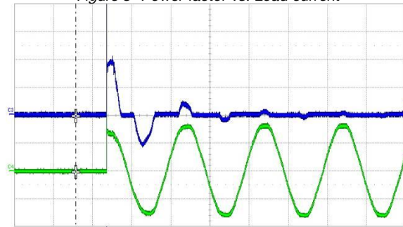
Figure 5- Inrush current, V_{in} = 230\text{Vac} , 90^\circ CH4: V_{in} (200V/div), CH3: I_n (20A/div)
