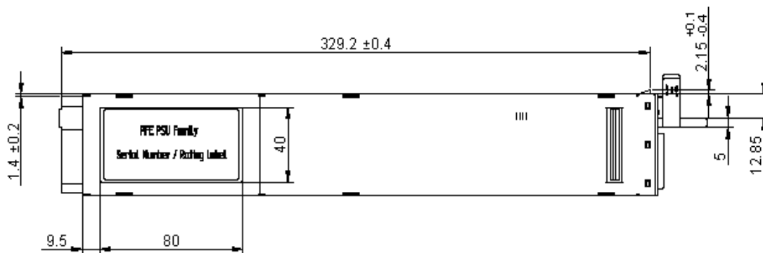
Figure 44 - Top View
