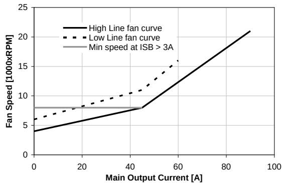
Figure 39 - Fan speed vs. main output load for PFE1100-12-054NA
