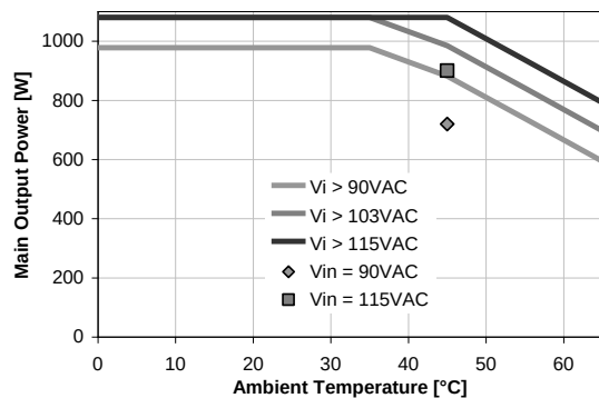
Figure 41 - Thermal derating for PFE1100-12-054NA
