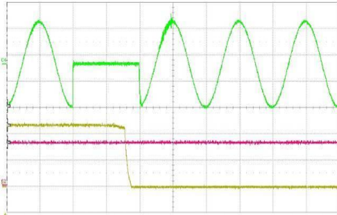
Figure 13- AC drop out 20 ms (10ms/div) CH1: V_1 (5V/div) CH2: V_{SB} (2V/div) CH4: V_n (200V/div)
