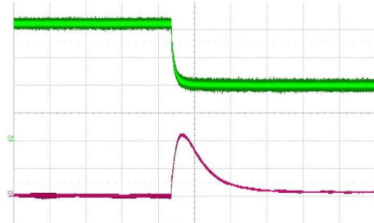
Figure 18 - Load transient V_1 , 85 to 40A (500μs/div) CH2: V_1 (200mV/div) CH4: I_1 (20A/div)
