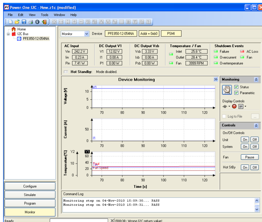
Figure 37 - Monitoring dialog of the I²C Utility
