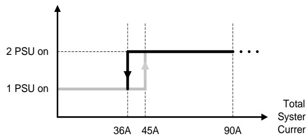
Figure 30 - Hot-standby enable/disable current thresholds
