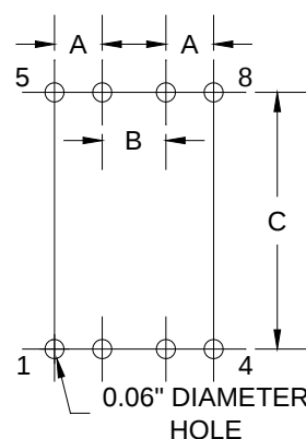
Board Layout
