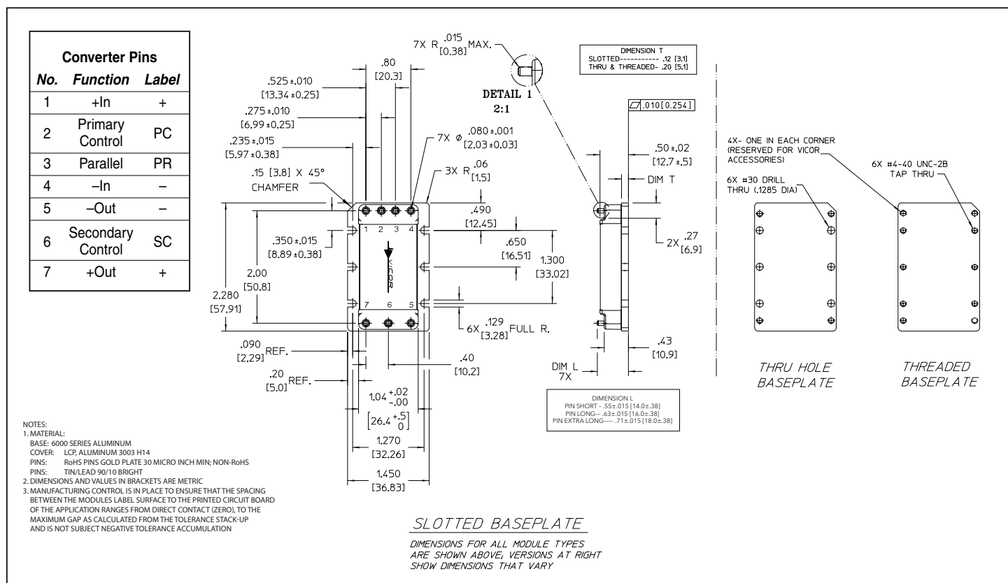
Figure 13 — Module outline
