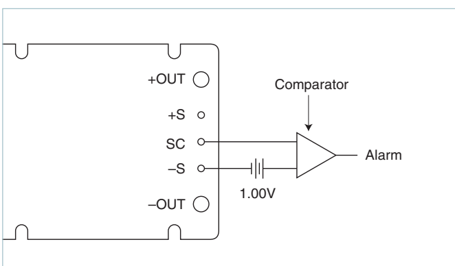
Figure 7 — Secondary side on-state indicator
