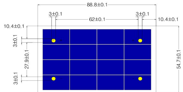
Back-side View
