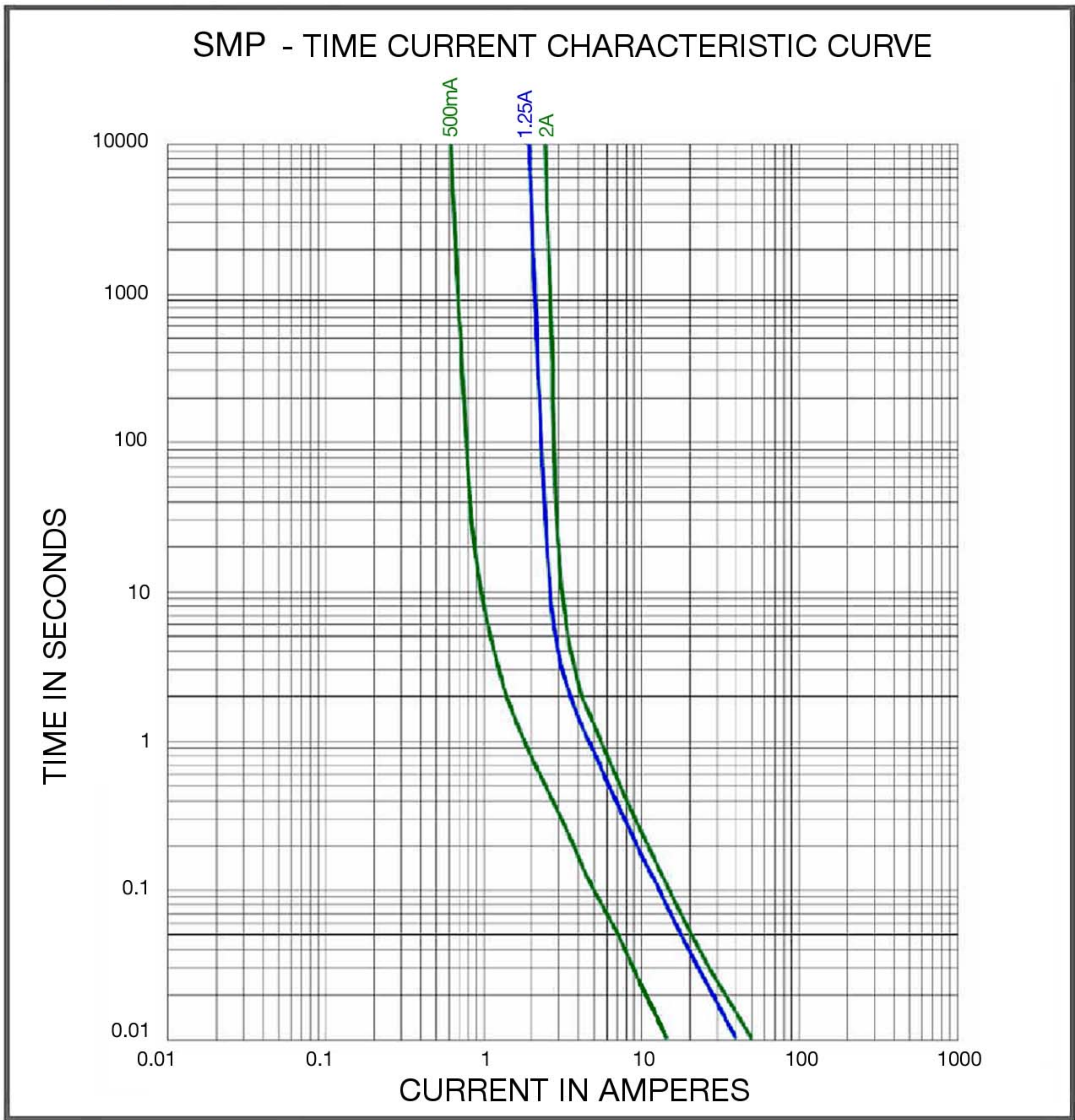
Average Time Current Curve
