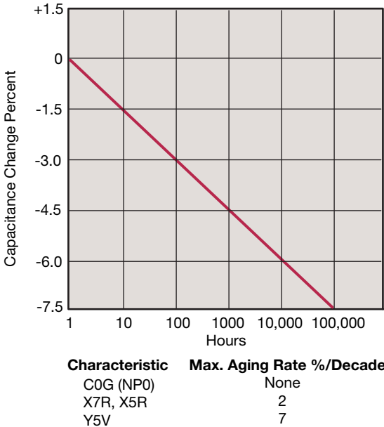
Typical Curve of Aging Rate X7R
