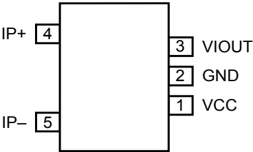
Pin-out Diagram
