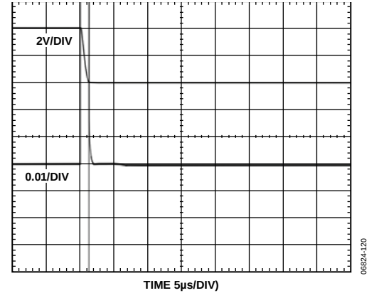
Figure 17. Settling Time (Falling)
