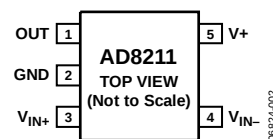
Figure 3. Pin Configuration
