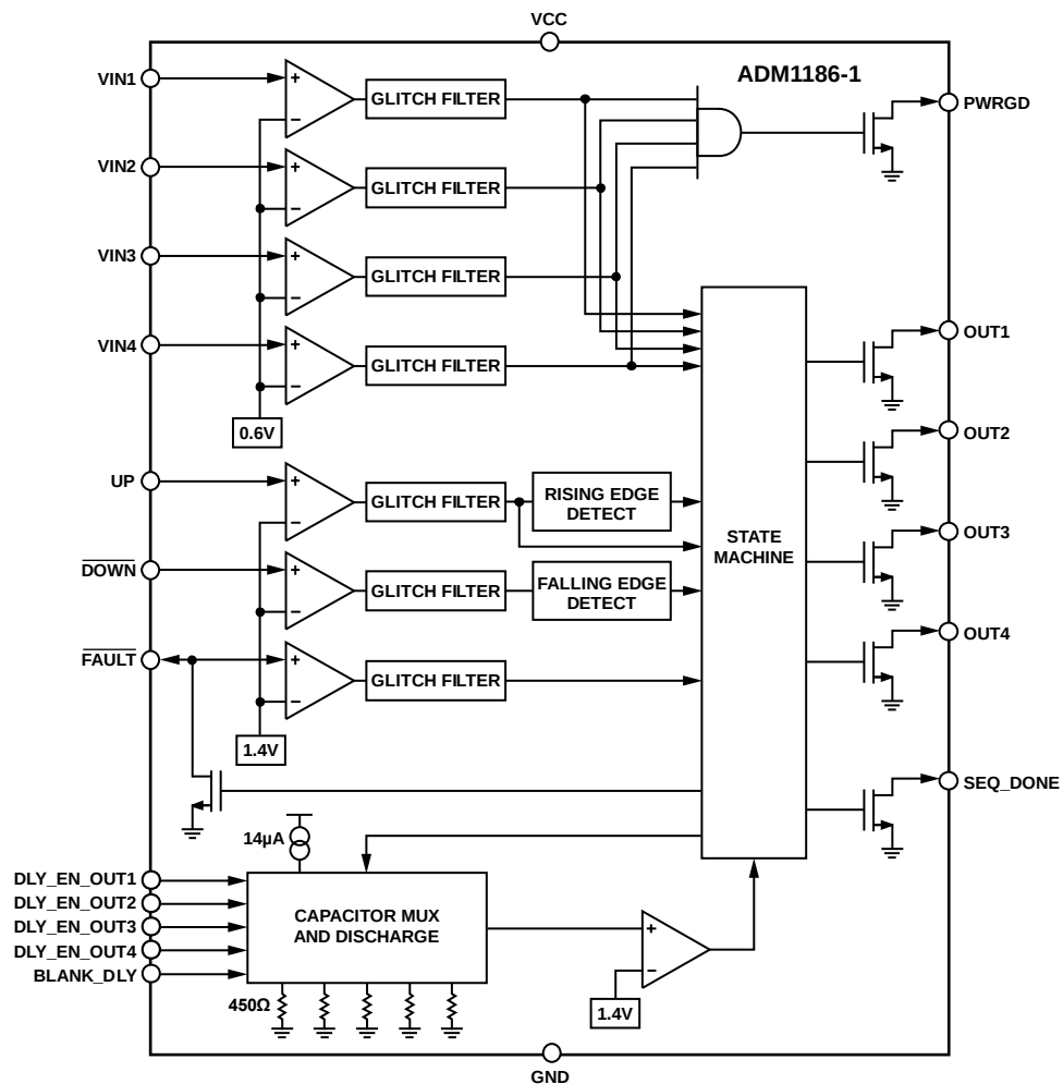
Figure 29. Functional Block Diagram of the ADM1186-1
