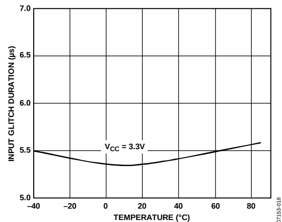
Figure 16. FAULT Input Glitch Immunity vs. Temperature
