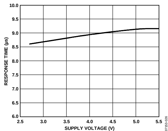
Figure 24. UP, \overline{\text{DOWN}} , UP/ \overline{\text{DOWN}} to \overline{\text{FAULT}} , OUTx Low Response Time vs. Supply Voltage
