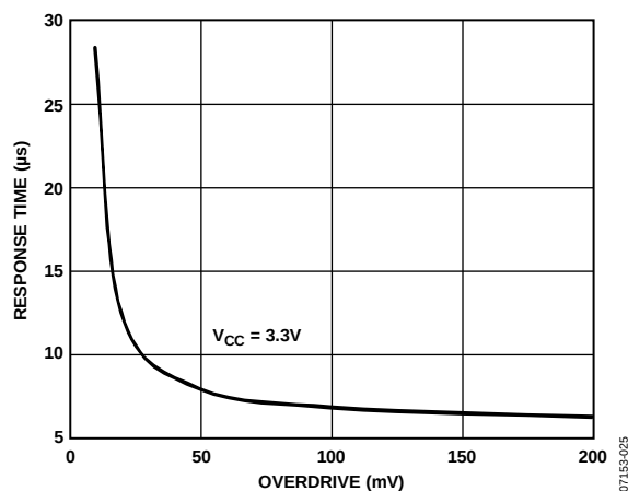
Figure 23. VINx to \overline{\text{FAULT}} , OUTx Low Response Time vs. Input Overdrive
