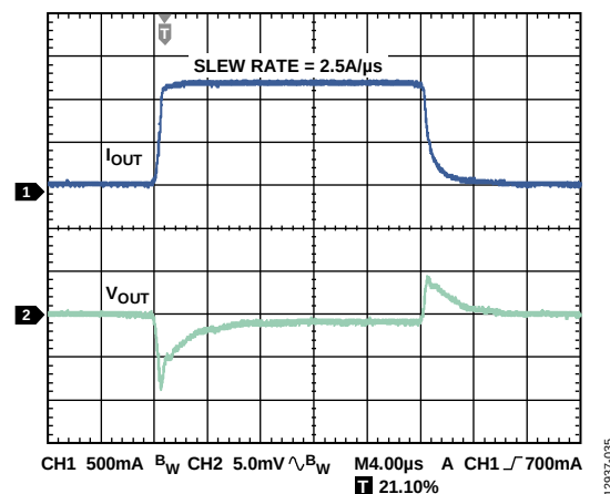
Figure 33. Load Transient Response, I_{LOAD} = 100mA to 1.2 A, V_{OUT} = 3.3V , V_{IN} = 4.0V , Channel 1 = I_{OUT} , Channel 2 = V_{OUT}
