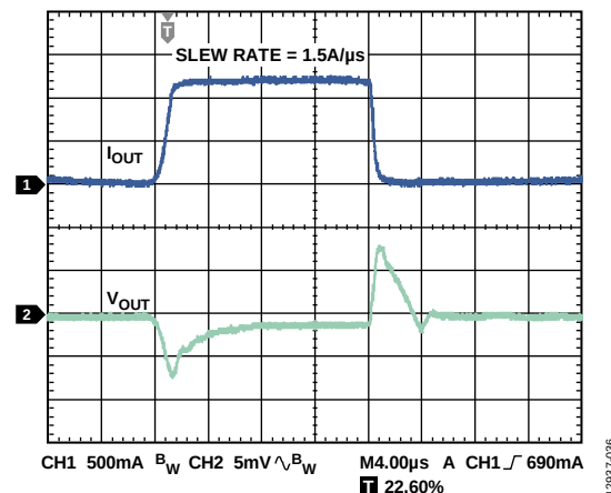
Figure 34. Load Transient Response, I_{LOAD} = 100mA to 1.2 A, V_{OUT} = 3.3V , V_{IN} = 4.0V , C_{OUT} = 22\mu F , Channel 1 = I_{OUT} , Channel 2 = V_{OUT}
