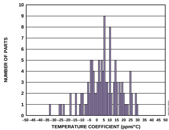
Figure 3. Temperature Coefficient, V_{OUT} = 0.5\text{ V}
