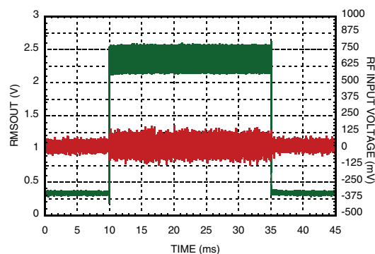
Figure 11. Residual Ripple for 1900 MHz GSM6C @ SCI=0011
