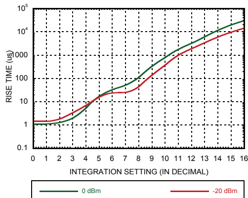
Figure 5. Rise Settling Time [3] vs. SCI Setting over Input Power
