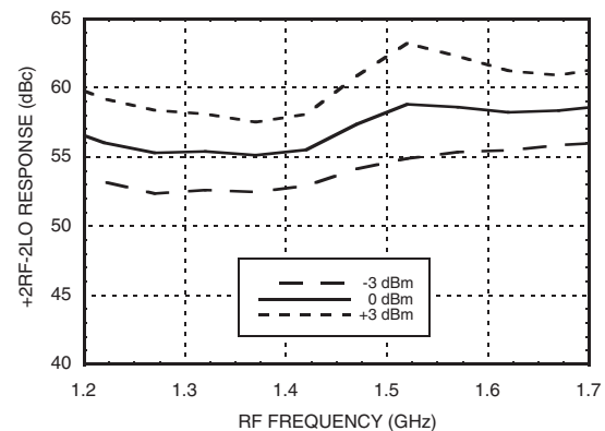
+2RF -2LO Response vs. LO Drive [2] [4]
