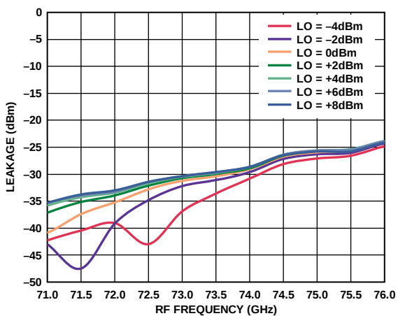
Figure 67. 6x LO Leakage at RFOUT vs. RF Frequency at Various LO Powers, I_{FIN} = 5 dBm, IF = 1000 MHz, USB
