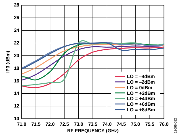
Figure 51. Input IP3 vs. RF Frequency at Various LO Powers, I_{FIN} = 5 dBm, IF = 500 MHz, USB
