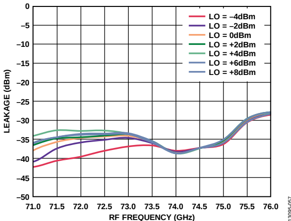
Figure 56. 6x LO Leakage at RFOUT vs. RF Frequency at Various LO Powers, I_{FIN} = 5 \text{ dBm} , IF = 500 \text{ MHz} , USB
