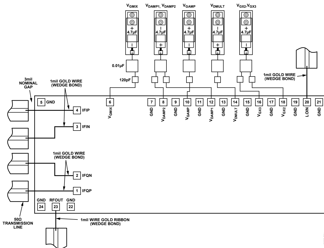
Figure 82. Assembly Diagram
