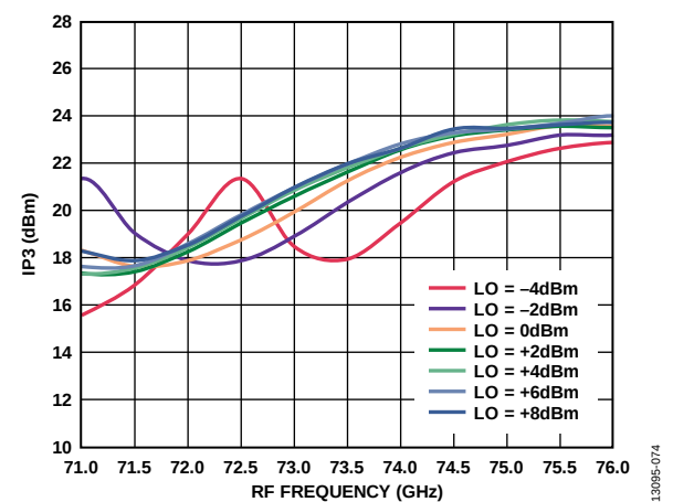
Figure 73. Input IP3 vs. RF Frequency at Various LO Powers, I_{FIN} = 5 dBm, IF = 2000 MHz, USB
