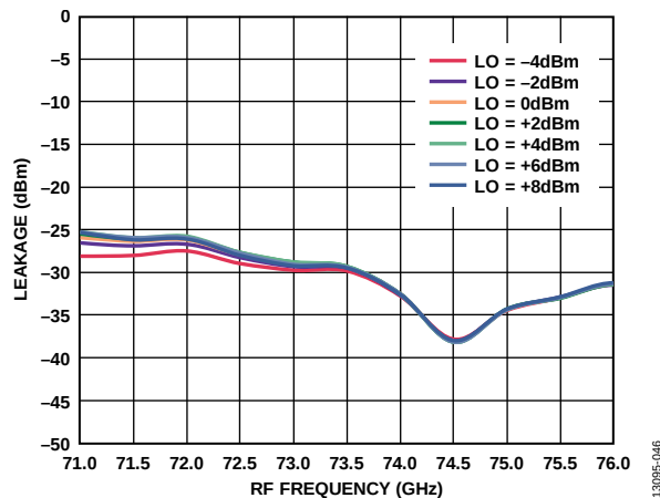
Figure 45. 6x LO Leakage at RFOUT vs. RF Frequency at Various LO Powers, I_{FIN} = 5 \text{ dBm} , IF = 2000 \text{ MHz} , LSB
