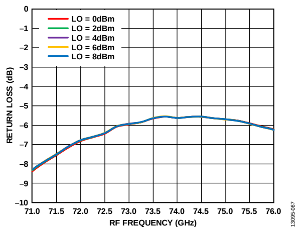
Figure 23. RF Port Return Loss vs. RF Frequency at Various LO Powers, RFIN = -10 dBm, LO = 12 GHz
