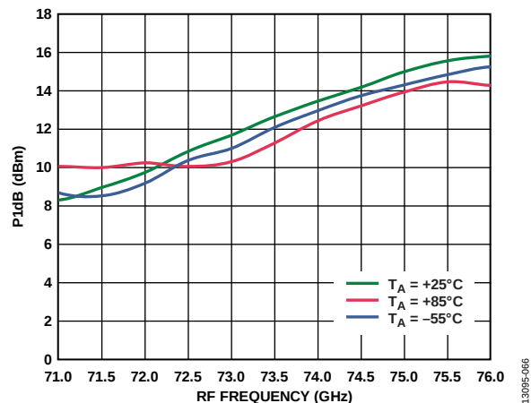
Figure 65. Input P1dB vs. RF Frequency at Various Temperatures, LO = 2 dBm, IF = 1000 MHz, USB
