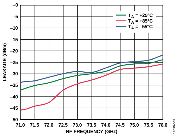
Figure 64. 6x LO Leakage at RFOUT vs. RF Frequency at Various Temperatures, I_{FIN} = 5 dBm, LO = 2 dBm, IF = 1000 MHz, USB
