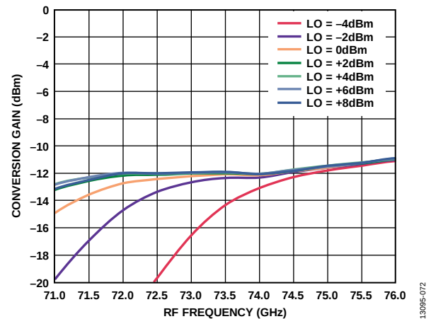
Figure 71. Conversion Gain vs. RF Frequency at Various LO Powers, I_{FIN} = -8 dBm, IF = 2000 MHz, USB
