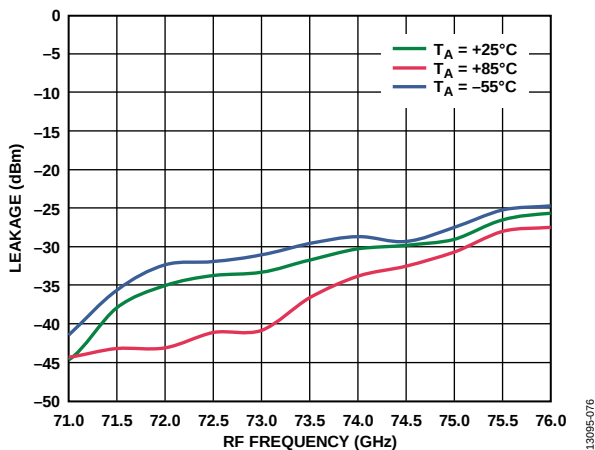
Figure 75. 6x LO Leakage at RFOUT vs. RF Frequency at Various Temperatures, I_{FIN} = 5 dBm, LO = 2 dBm, IF = 2000 MHz, USB
