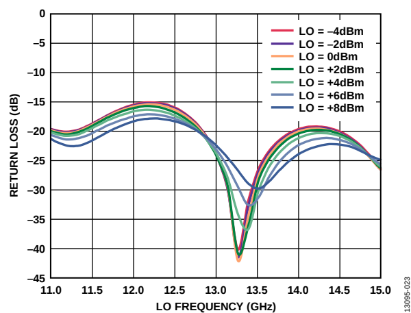
Figure 22. LO Port Return Loss vs. LO Frequency at Various LO Powers
