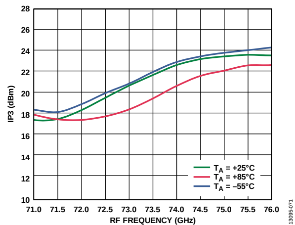
Figure 70. Input IP3 vs. RF Frequency at Various Temperatures, I_{FIN} = 5 dBm, LO = 2 dBm, IF = 2000 MHz, USB
