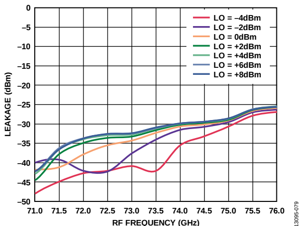
Figure 78. 6x LO Leakage at RFOUT vs. RF Frequency at Various LO Powers, I_{FIN} = 5 dBm, IF = 2000 MHz, USB
