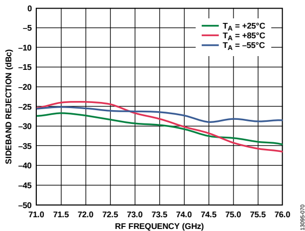
Figure 69. Sideband Rejection vs. RF Frequency at Various Temperatures, I_{FIN} = -8 dBm, LO = 2 dBm, IF = 2000 MHz, USB
