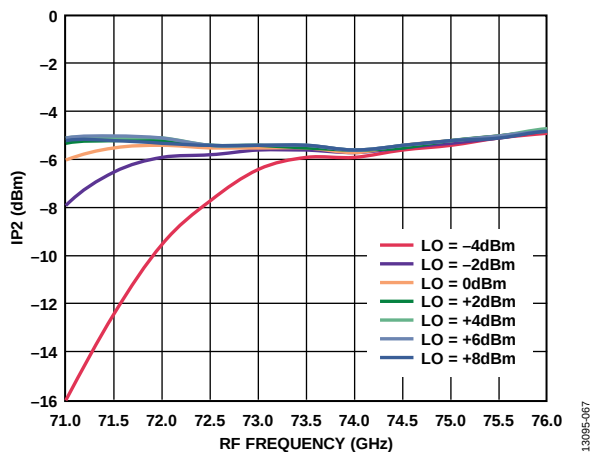
Figure 66. Input IP2 vs. RF Frequency at Various LO Powers, I_{FIN} = 5 dBm, IF = 1000 MHz, USB
