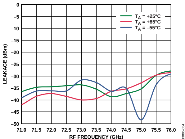
Figure 53. 6x LO Leakage at RFOUT vs. RF Frequency at Various Temperatures, I_{FIN} = 5 \text{ dBm} , LO = 2 \text{ dBm} , IF = 500 \text{ MHz} , USB
