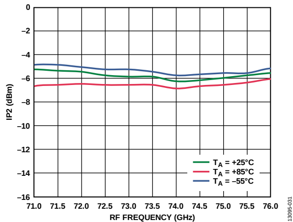
Figure 30. Input IP2 vs. RF Frequency at Various Temperatures, I_{FIN} = 5 \text{ dBm} , LO = 2 \text{ dBm} , IF = 500 \text{ MHz} , LSB
