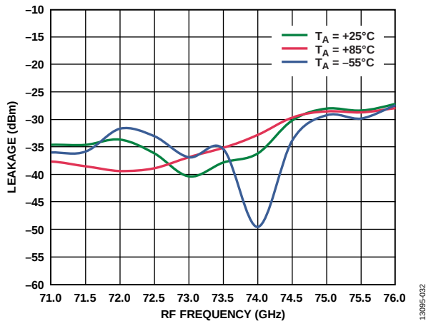
Figure 31. 6x LO Leakage at RFOUT vs. RF Frequency at Various Temperatures, I_{FIN} = 5 \text{ dBm} , LO = 2 \text{ dBm} , IF = 500 \text{ MHz} , LSB
