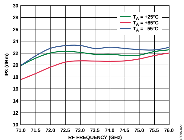
Figure 26. Input IP3 vs. RF Frequency at Various Temperatures, IF_{IN} = 5 dBm, LO = 2 dBm, IF = 500 MHz, LSB
