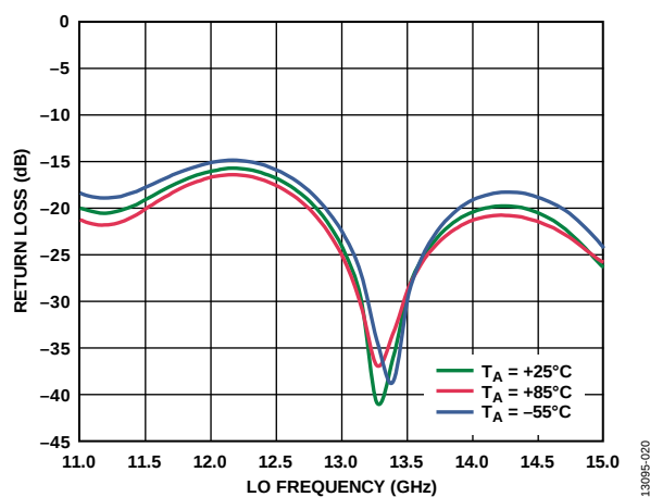
Figure 19. LO Port Return Loss vs. LO Frequency at Various Temperatures, LO = 2 dBm
