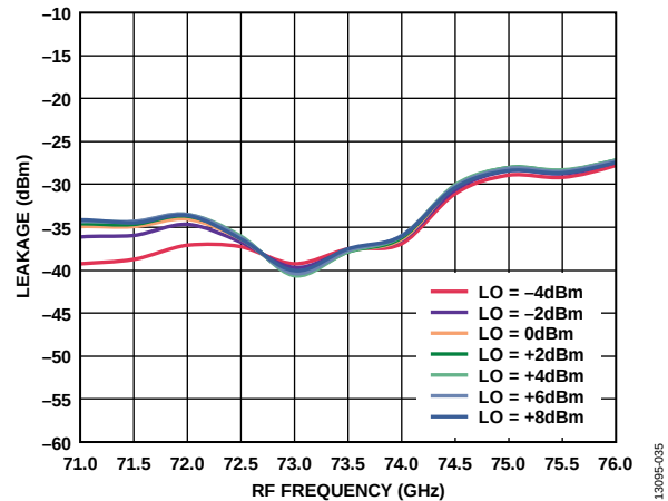
Figure 34. 6x LO Leakage at RFOUT vs. RF Frequency at Various LO Powers, I_{FIN} = 5 \text{ dBm} , IF = 500 \text{ MHz} , LSB
