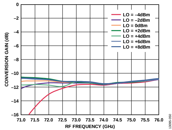
Figure 49. Conversion Gain vs. RF Frequency at Various LO Powers, I_{FIN} = -8 dBm, IF = 500 MHz, USB
