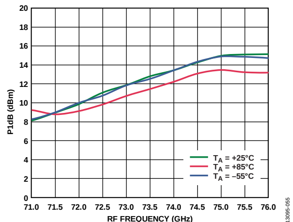
Figure 54. Input P1dB vs. RF Frequency at Various Temperatures, LO = 2 \text{ dBm} , IF = 500 \text{ MHz} , USB
