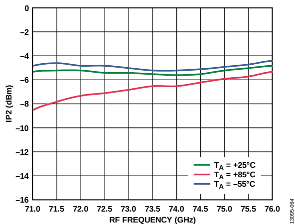
Figure 63. Input IP2 vs. RF Frequency at Various Temperatures, I_{FIN} = 5 dBm, LO = 2 dBm, IF = 1000 MHz, USB
