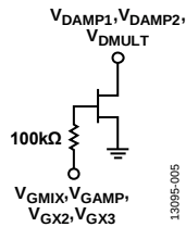
Figure 5. VGMIX, VDAMP1, VDAMP2, VDMULT, VGAMP, VGX2, VGX3 Interface
