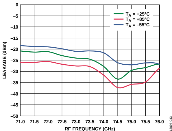
Figure 42. 6x LO Leakage at RFOUT vs. RF Frequency at Various Temperatures, I_{FIN} = 5 \text{ dBm} , LO = 2 \text{ dBm} , IF = 2000 \text{ MHz} , LSB
