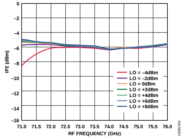
Figure 33. Input IP2 vs. RF Frequency at Various LO Powers, I_{FIN} = 5 \text{ dBm} , IF = 500 \text{ MHz} , LSB
