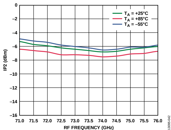
Figure 41. Input IP2 vs. RF Frequency at Various Temperatures, I_{FIN} = 5 \text{ dBm} , LO = 2 \text{ dBm} , IF = 2000 \text{ MHz} , LSB
