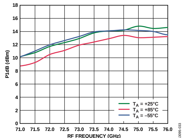
Figure 32. Input P1dB vs. RF Frequency at Various Temperatures, LO = 2 \text{ dBm} , IF = 500 \text{ MHz} , LSB
