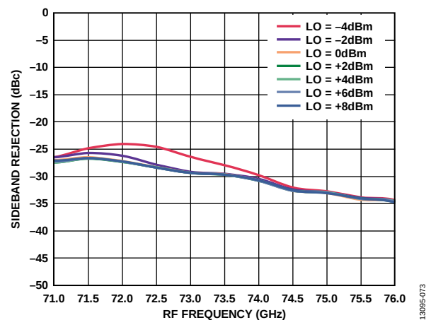
Figure 72. Sideband Rejection vs. RF Frequency at Various LO Powers, I_{FIN} = -8 dBm, IF = 2000 MHz, USB
