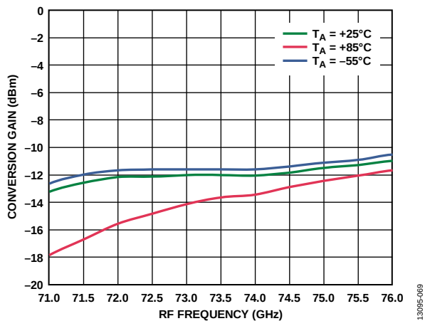
Figure 68. Conversion Gain vs. RF Frequency at Various Temperatures, I_{FIN} = -8 dBm, LO = 2 dBm, IF = 2000 MHz, USB
