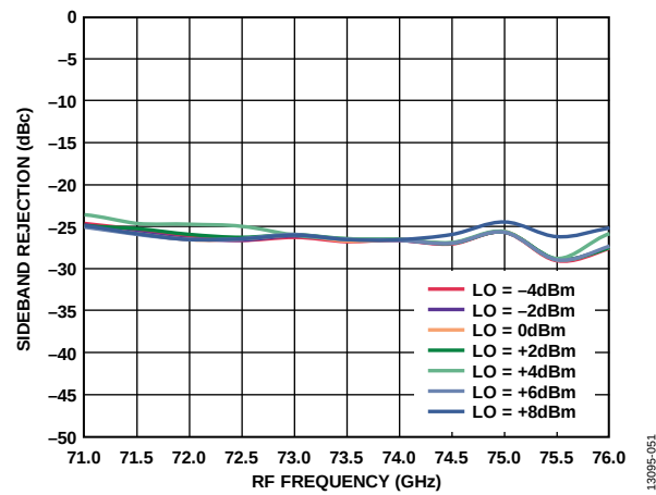
Figure 50. Sideband Rejection vs. RF Frequency at Various LO Powers, I_{FIN} = -8 dBm, IF = 500 MHz, USB
