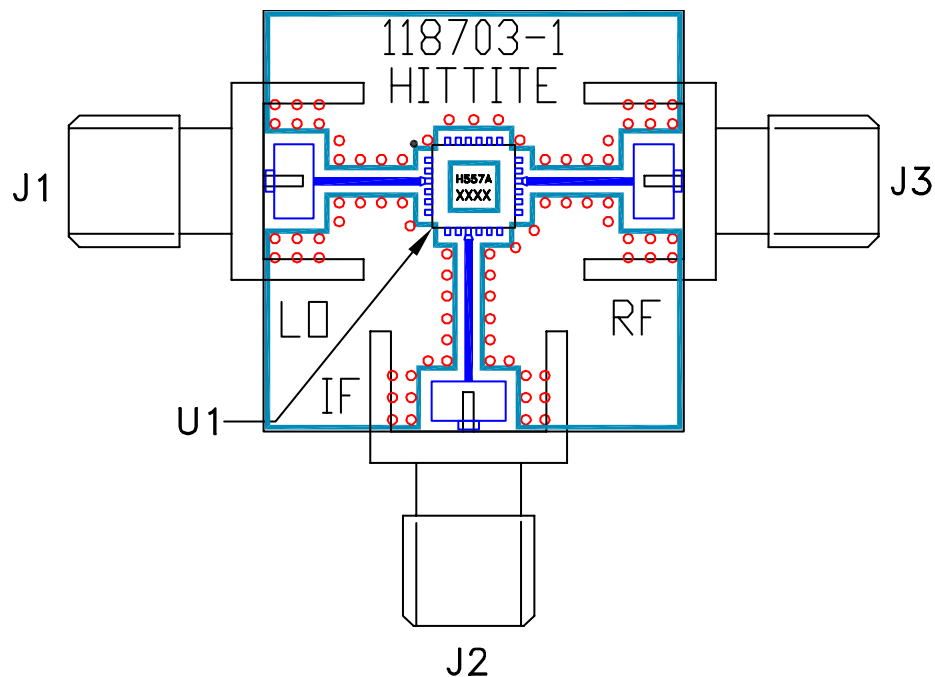
Figure 83. Evaluation Printed Circuit Board (PCB)
