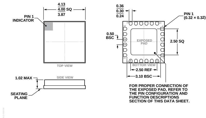
Figure 84. 24-Terminal Ceramic Leadless Chip Carrier [LCC] (E-24-1)
