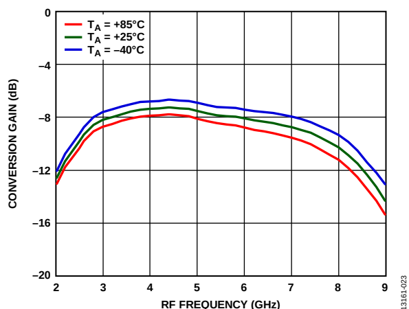
Figure 29. Conversion Gain vs. RF Frequency at Various Temperatures, LO Drive = 15 dBm
