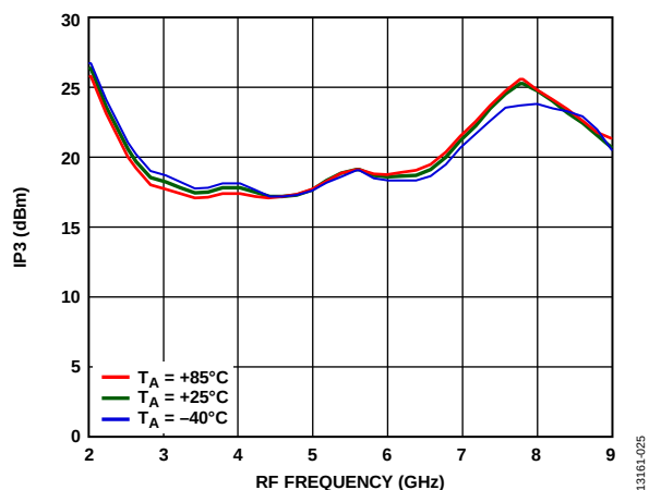
Figure 30. Input IP3 vs. RF Frequency at Various Temperatures, LO Drive = 15 dBm
