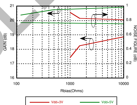
Gain, Noise Figure vs. Rbias @ 2100 MHz
