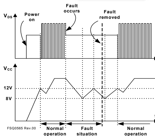
Figure 29. Auto Restart Protection Waveforms
