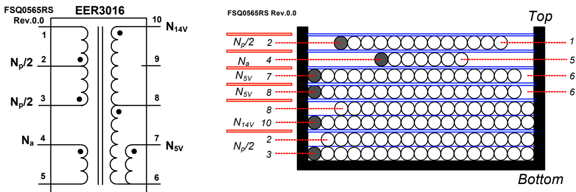
Figure 40. Transformer Schematic Diagram of FSQ0565RS
