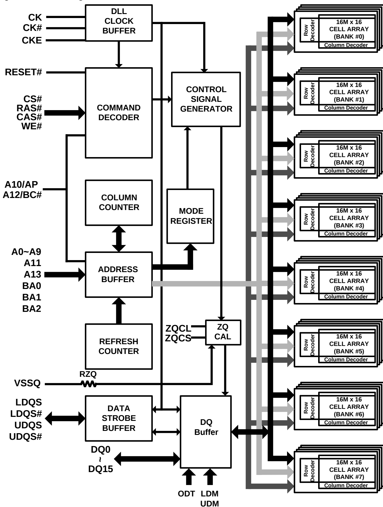
Figure 2. Block Diagram
