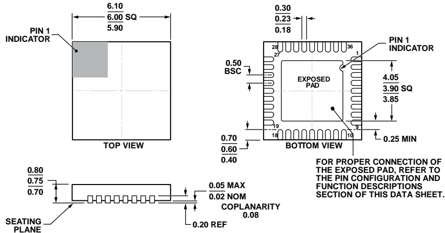
Figure 47. 36-Lead Lead Frame Chip Scale Package [LFCSP_WQ] 6 mm x 6 mm Body, Very Very Thin Quad (CP-36-3) Dimensions shown in millimeters
