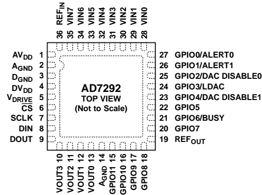
Figure 3. Pin Configuration
